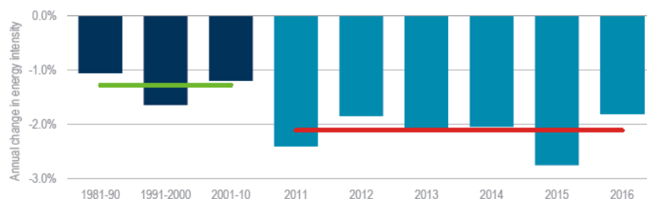
Figure 1. Annual changes in global primary energy intensity, 1981–2016 (US dollars (USD), 2016).
