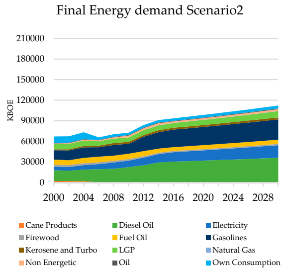
Figure 11. Final energy demand scenarios.
