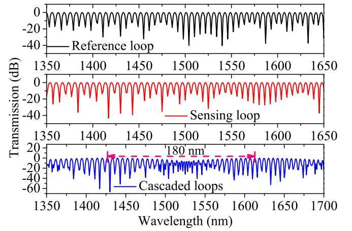
Fig. 6. Simulated transmission spectrum of the reference-, sensing-loop and the cascaded loops from top to bottom. FSRs of the reference- and sensing-loop are nearly the same of \sim 6 nm, FSR_{Env} of the cascaded loops is \sim 180 nm for the upper envelope. Magnification can reach to 30.
