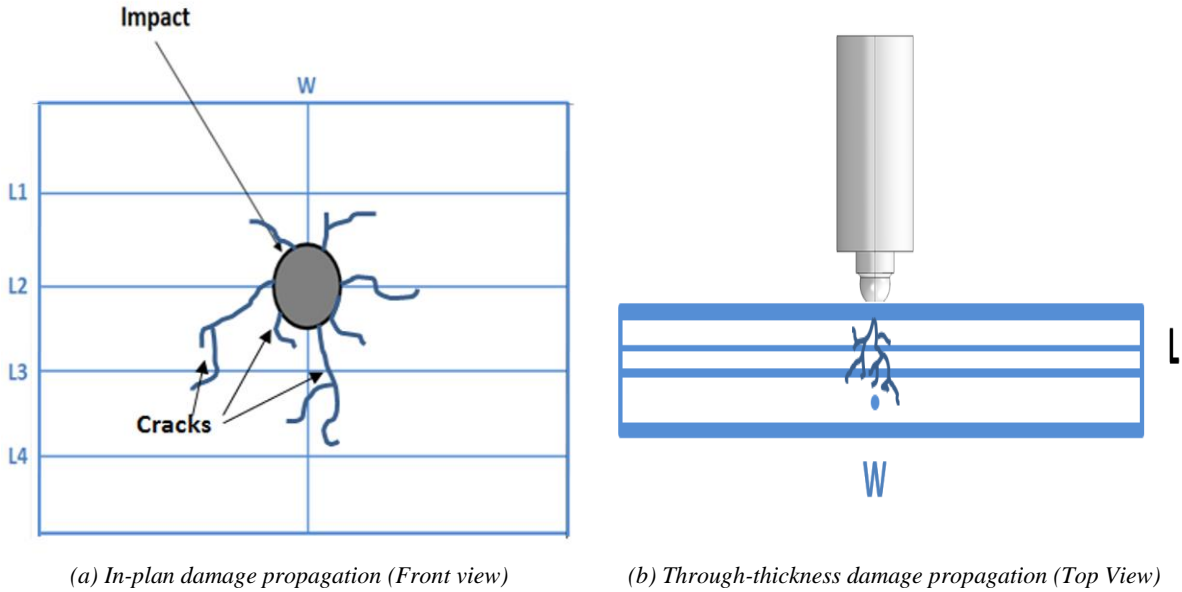
Figure 11: Overall fracture and damage propagation during the impact of composite plate.
