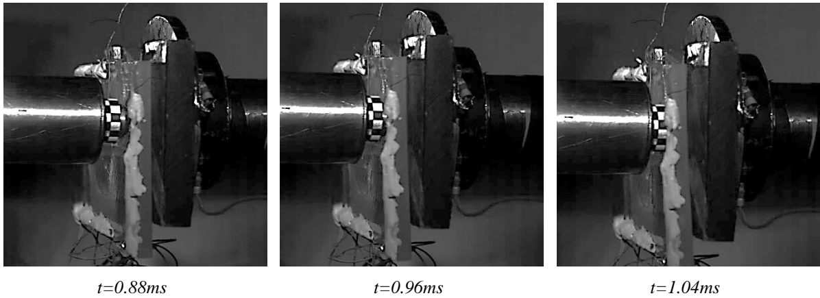
Figure 12: Real-time high-speed photographs of dynamic impact test performed at v=6.5 m/s on the composite sample.
