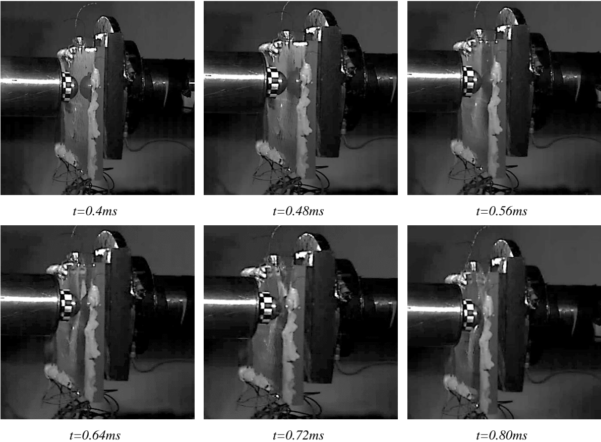
Figure 11: Overall fracture and damage propagation during the impact of composite plate.
