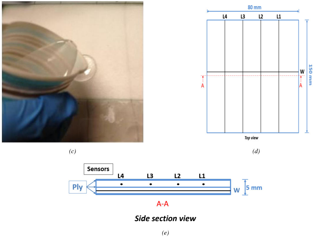
Figure 3: (a)-(c) Composite sample preparation process with integration of Nylon/Ag fiber sensors (d)-(e) Geometric parameters of the samples and placement of Nylon/Ag fiber sensor in each position correspondingly.
