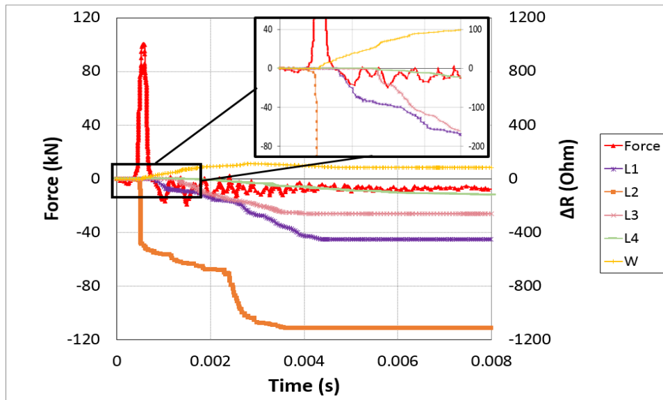
Figure 17: In-situ monitoring in the composite sample by Nylon/Ag fiber sensor subjected to dynamic impact at velocity 6.5 m/s
