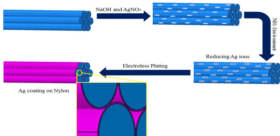
Figure 1: Manufacturing process of Nylon/Ag fiber sensor
