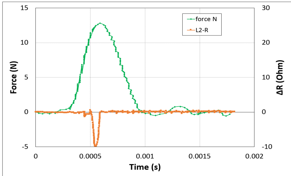
Figure 15: In-situ detection of deformation in the composite sample under dynamic impact at v= 2.5 m/s by Nylon/Ag fiber sensor.
