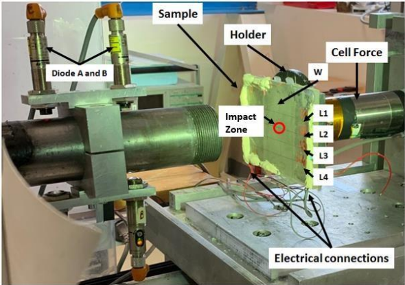
Figure 4: Experimental setup to calculate the Gauge Factor of the fiber sensor.
