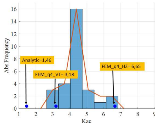
Fig. 14. Experimental Absolute Frequency of K_{AC} for motorette with q=4 at 1000Hz.
