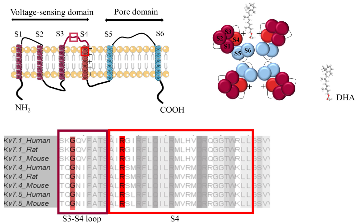
FIGURE 4 Putative \omega -3 polyunsaturated fatty acid (PUFA) binding domains in K_v7.1 , K_v7.4 and K_v7.5 are highly conserved across humans, rats and mice. The tertiary and quaternary structure of K_v7.1 inferred from the crystal structure of K_v1.2 (Smith, Vanoye, George, Meiler, & Sanders, 2007). This channel is a tetramer consisting of four identical monomers. Each monomer consists of 6 subunits: subunits S1-S4 form the voltage sensing domain and subunits S5-S6 form the pore domain. The outermost positive charge of S4 is an arginine (R228), marked in a bright red square and contributes to docosahexaenoic acid (DHA) affinity. This essential residue is conserved across species and channel subtype. The non-polar glycine in the S3-S4 loop (G219), also marked in a dark red square, which is also essential for DHA affinity and is also highly conserved. Servier Medical Art by Servier is licensed under a Creative Commons Attribution 3.0 Unported License
