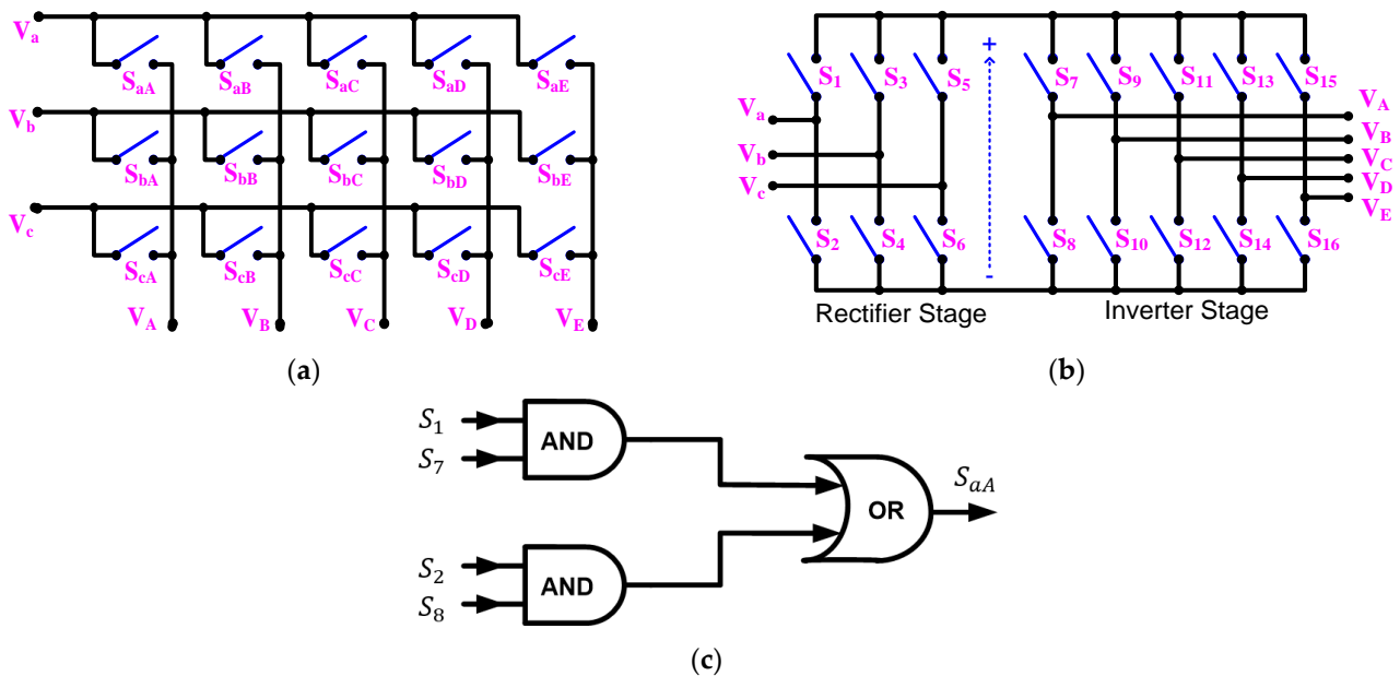
Figure 1. (a) Direct five-phase matrix converter (MC), (b) indirect five-phase MC and (c) transformation from an indirect to direct topology for switch S_{aA} .
