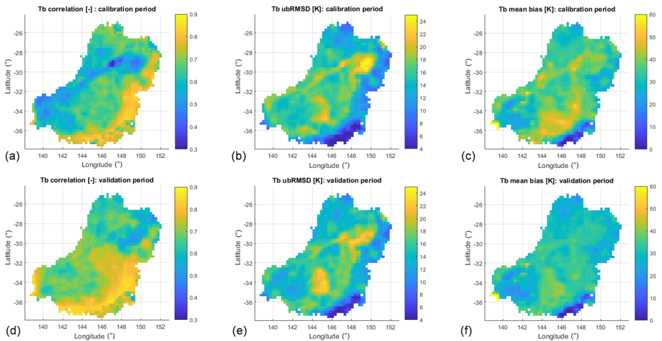
Figure 3. Performance and error metrics of SFX-simulated Tb using, as a reference, SMOS Tb. \rho coefficients (a, d), unbiased root mean square deviations (ubRMSD; b, e) and mean biases (c, f) between SFX–CMEM predictions and SMOS observations of Tb during the calibration (a–c) and the validation (d–f) periods.
