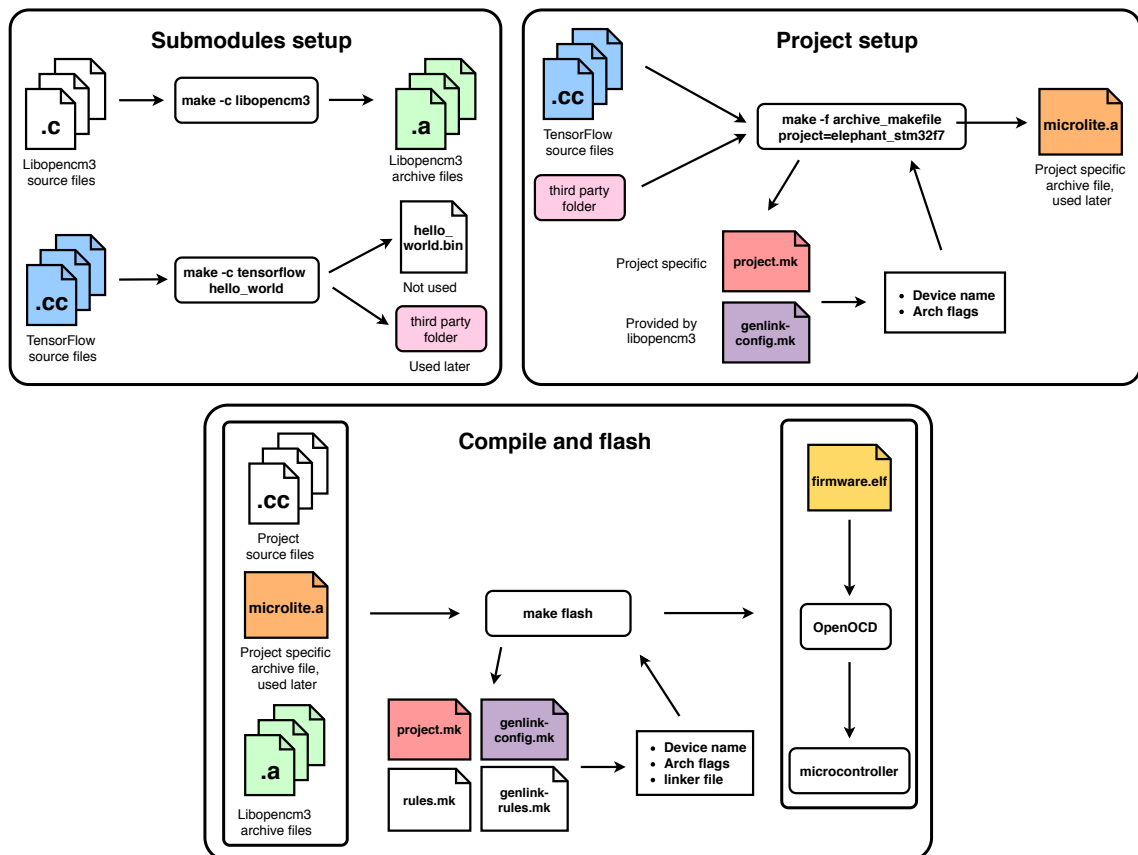
Figure 4.14: Build system of MicroML project.
