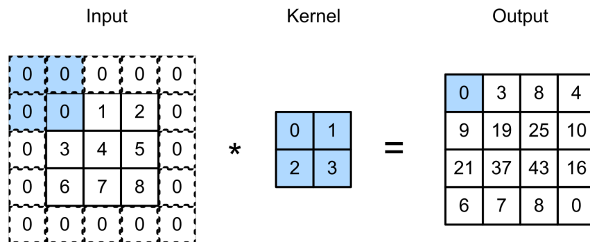
Figure 2.5: Dot product operation between filter and zero-padded input matrix. Image sources: [22]
