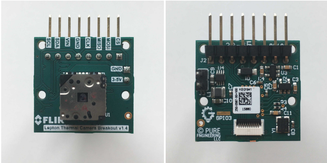
Figure 4.8: Front and back side of FLIR Lepton breakout board with thermal camera module inserted.
