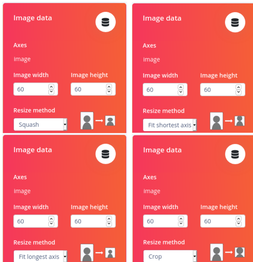
Figure 3.9: Different resizing methods
