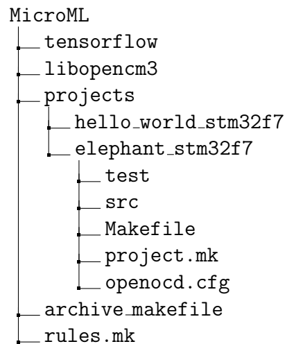
Figure 4.13: Directory structure of the MicroML project.
