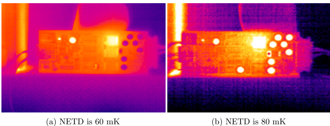
Figure 2.13: Comparison of images of the same object taken with cameras with different NETD values. Low NETD values are more appropriate for object recognition. Image source: MoviTherm [33]
