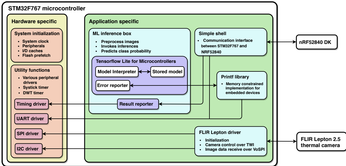
Figure 4.10: Architecture diagram of the firmware that is running on the STM32 microcontroller.
