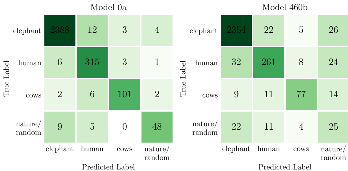
Figure 5.1: Confusion matrices of 0a model (left) and 460b model (right).
