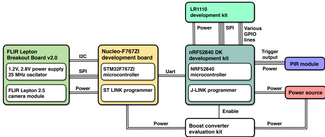
Figure 4.3: Hardware diagram of the embedded early warning system
