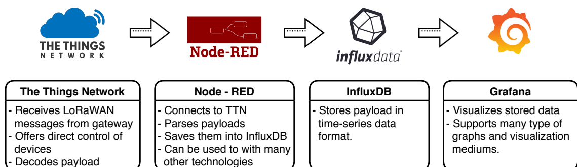
Figure 4.15: Server side flow of information. Icons source: [11]
