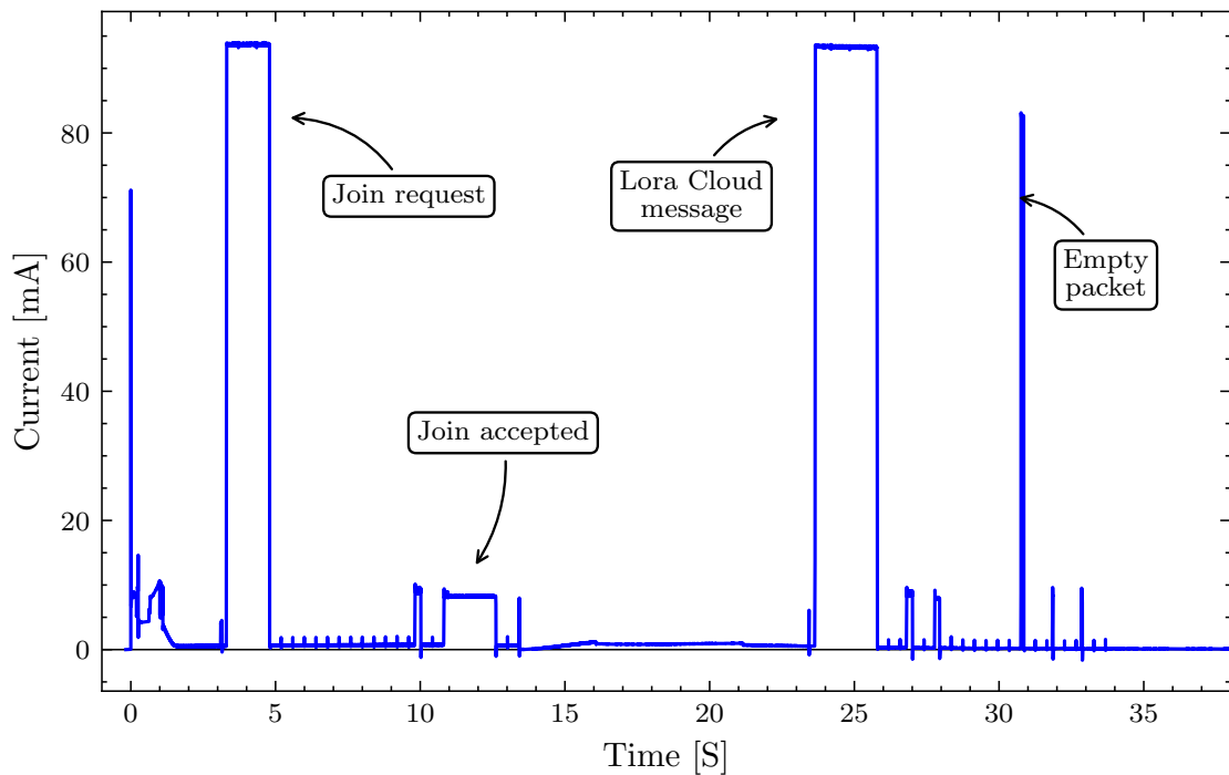
Figure 5.9: Current profile of the LoRaWAN join sequence.
