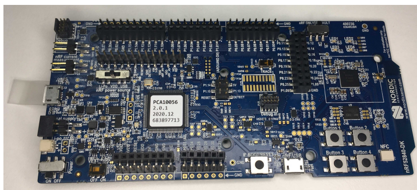
Figure 4.5: nRF52840DK development board
