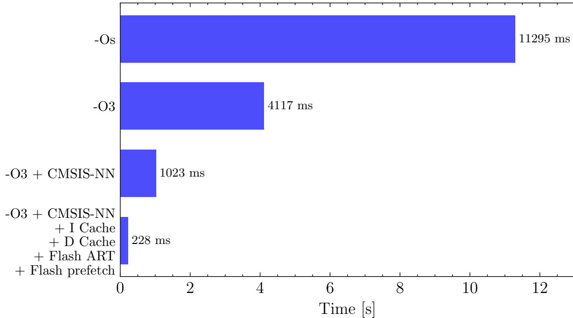
Figure 5.4: Inference time of the 0b model using different optimisations.
