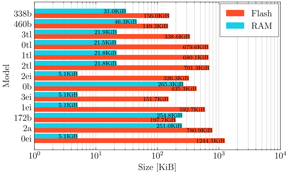
Figure 5.3: Comparison of Flash and RAM size of compiled example models.
