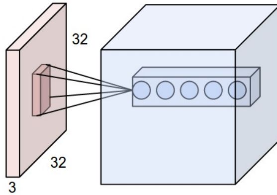
Figure 2.6: Convolutional layer with five different filters. Image sources: [22] [16]
