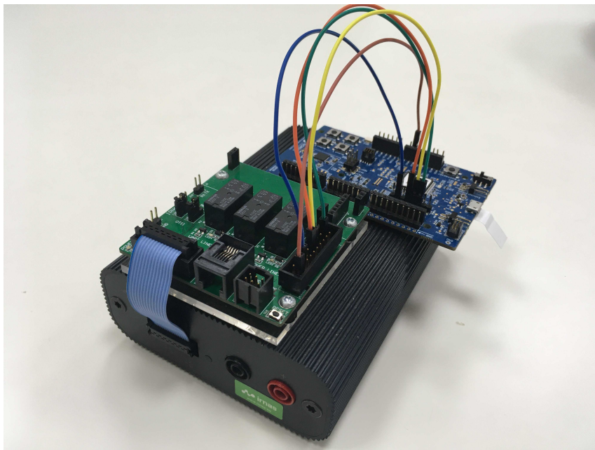
Figure 5.6: Otii Arc with nRF52832 DK and added measurement board made by IRNAS.
