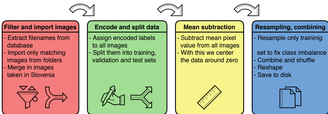
Figure 3.6: Image preprocessing pipeline. Icons source: [11]
