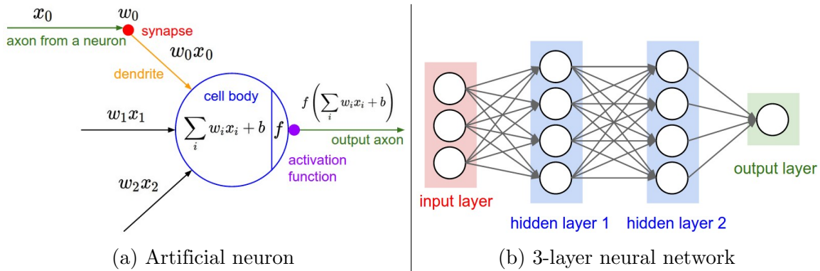
Figure 2.2: (a) Mathematical model of an artificial neuron, similarities with biological neurons can be seen. (b) Fully connected 3-layer neural network. Image source: [16]
