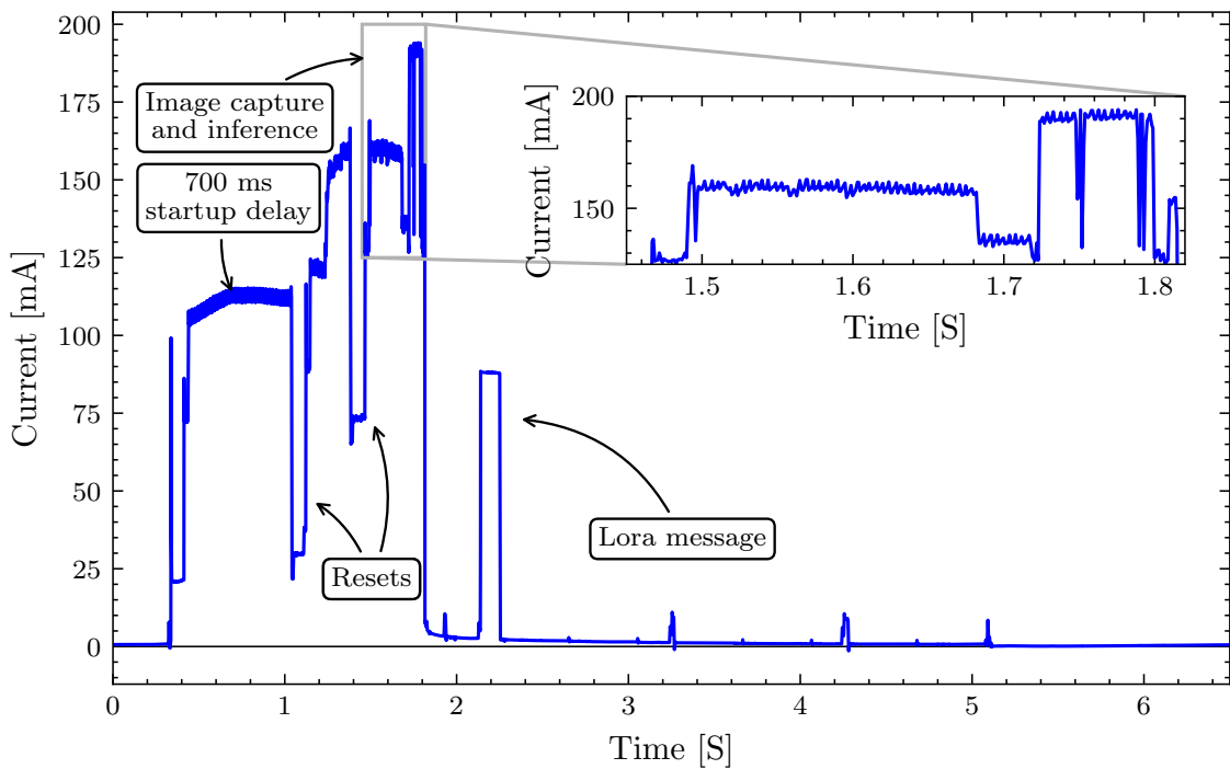
Figure 5.11: Current profile of image capture and inference procedure.
