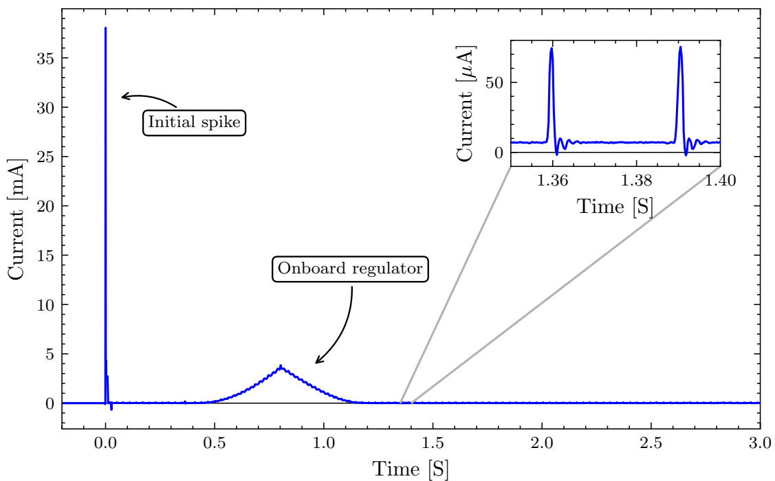
Figure 5.8: Current consumption of nRF52840 microcontroller in low-power state.
