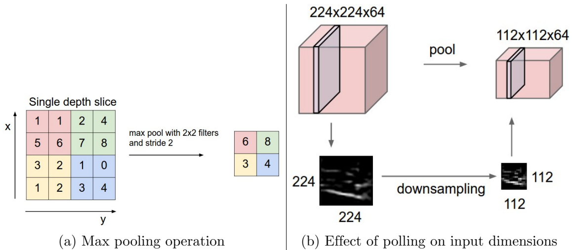
Figure 2.7: Pooling layer. Image source: [16]
