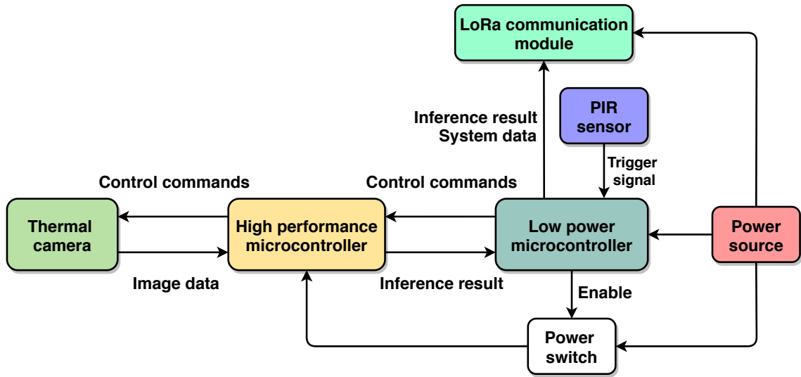
Figure 4.1: General block diagram of an embedded system
