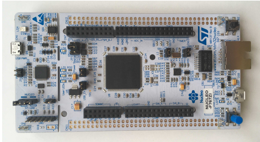
Figure 4.4: Nucleo-F767ZI development board
