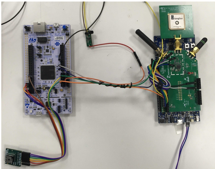
Figure 5.10: Device under test: nRF52840 DK with attached LR1110 shield, boost converter breakout board, Nucleo-F767ZI and FLIR Lepton camera.
