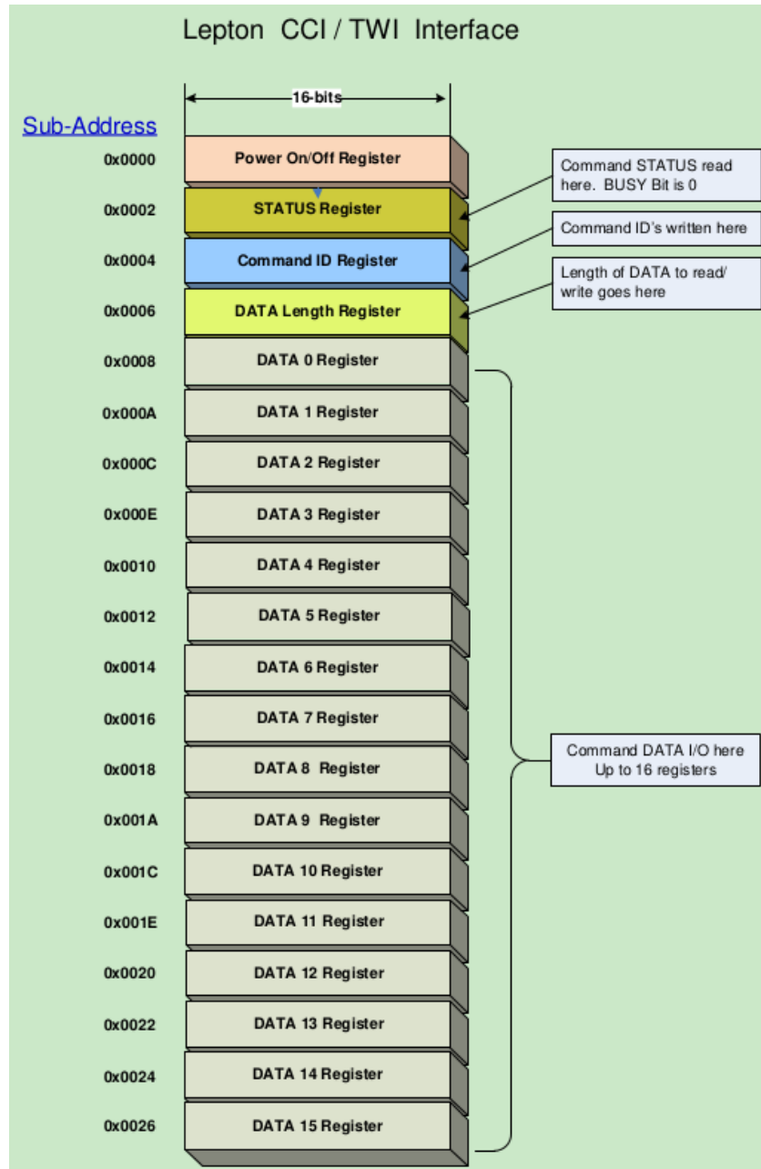
Figure 4.12: Command and control interface of an FLIR Lepton camera. Image source: [37]
