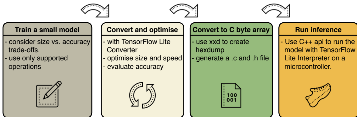
Figure 2.9: Workflow of preparing a ML model for an inference on a microcontroller. Icons source: [11]
