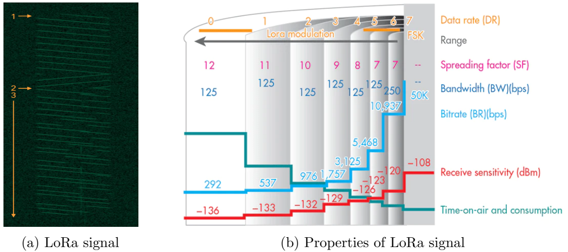
Figure 2.10: Lora signal (left) and different properties of LoRa with their effects on range, bit rate, receiver sensitivity, time on air and consumption (right). Image sources: [28] [29]
