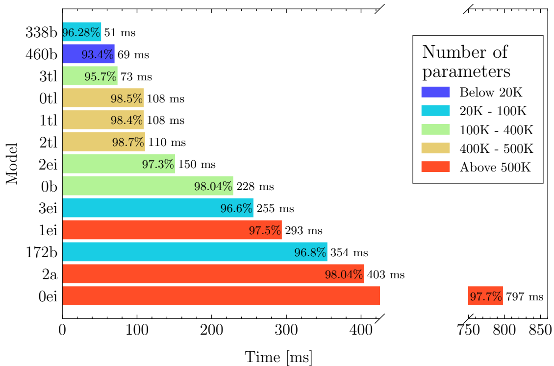
Figure 5.2: Comparison of time of inference of different models.
