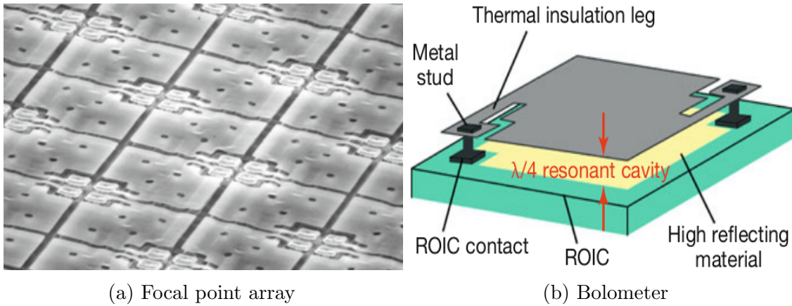
Figure 2.12: (a) Focal point array under electronic microscope. (b) Bolometer with \lambda/4 resonant cavity. Image source: Vollmer, Möllmann [31]
