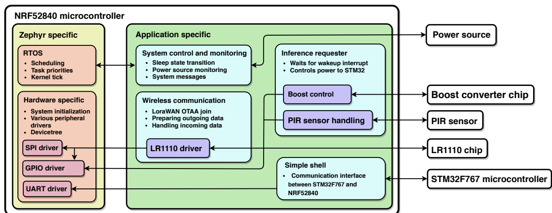
Figure 4.11: Architecture diagram of the firmware that is running on the nRF52840 microcontroller.
