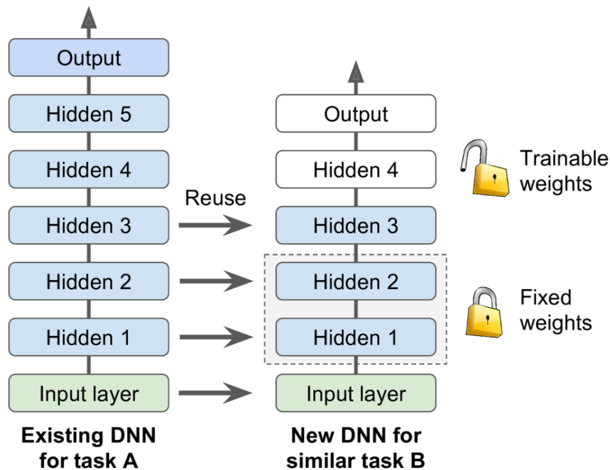
Figure 2.8: Transfer Learning. Image source: [14]
