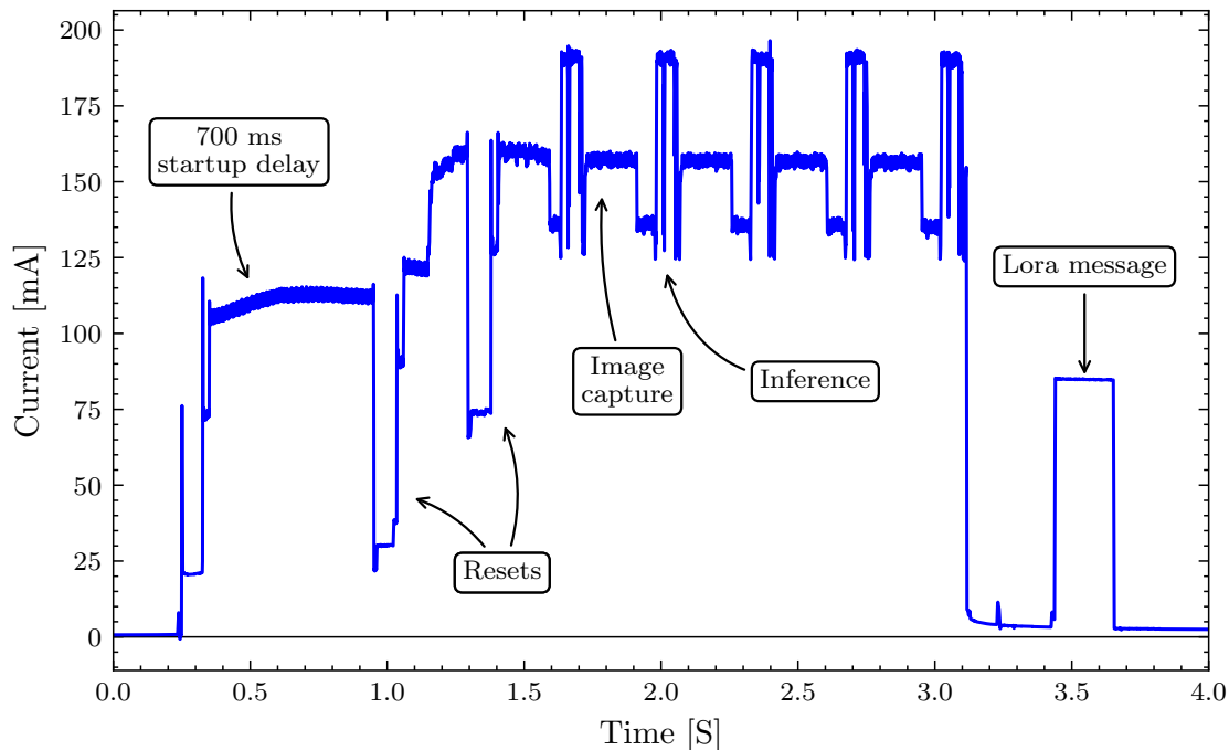
Figure 5.12: Current profile of image capture and inference procedure repeated 5 times.
