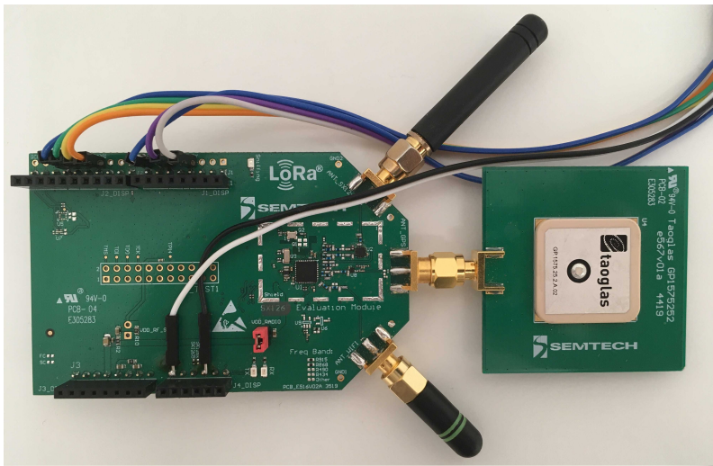
Figure 4.6: LR1110 development kit
