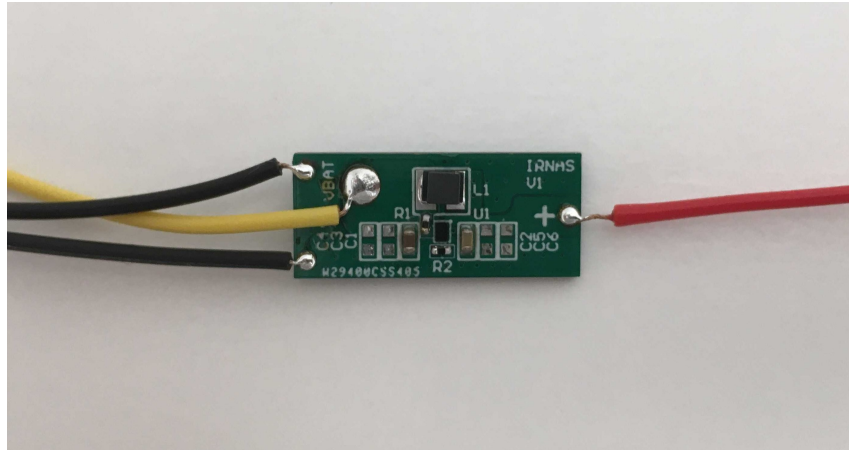
Figure 4.7: MAX17225ENT+T boost converter breakout board
