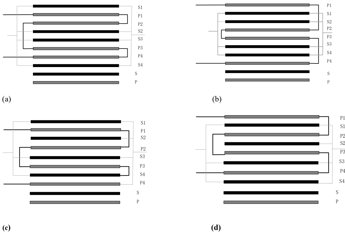
Fig. 3.5 Normally used kind of Crossing structure
