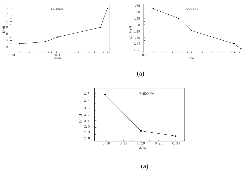
Fig. 3.4 (a) Relationship between leakage, AC resistance and spacing (b) Power in isolation layer and thickness
