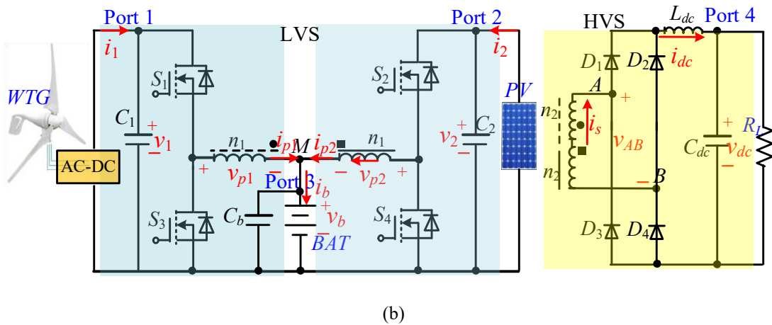
Fig. 4.3 the proposed four-port DC-DC converter
