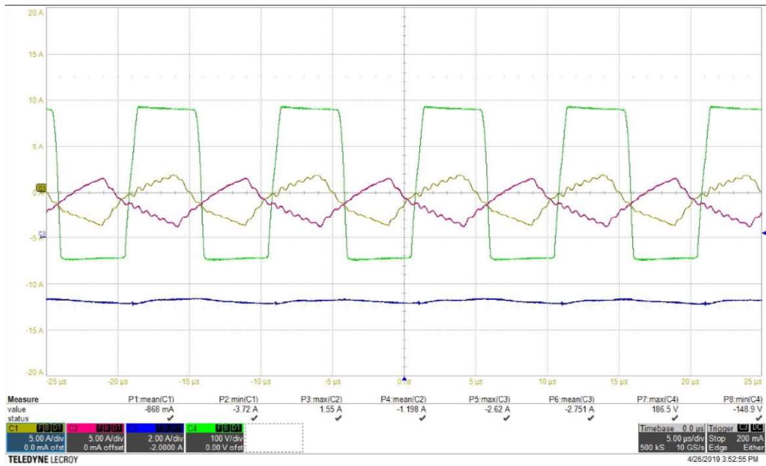
Fig. 5.5 Steady-state waveform of i_{p1} , i_{p2} , and v_{AB} . (a) charge mode (b) Discharge mode
