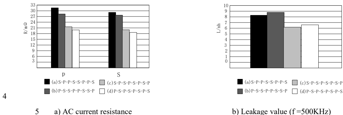
Fig. 3.7 Current and leakage value in different combination
