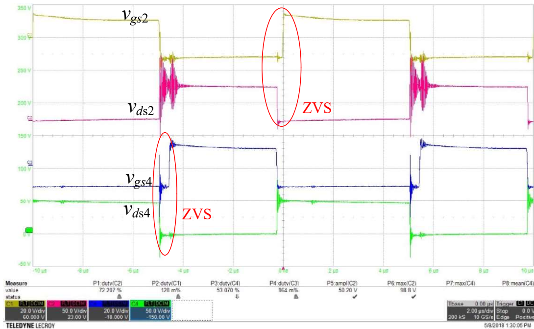
Fig. 5.6 Measured ZVS of switches S2 and S4.
