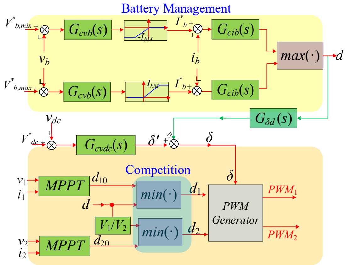
Fig. 4.7 Organization of controllers.
