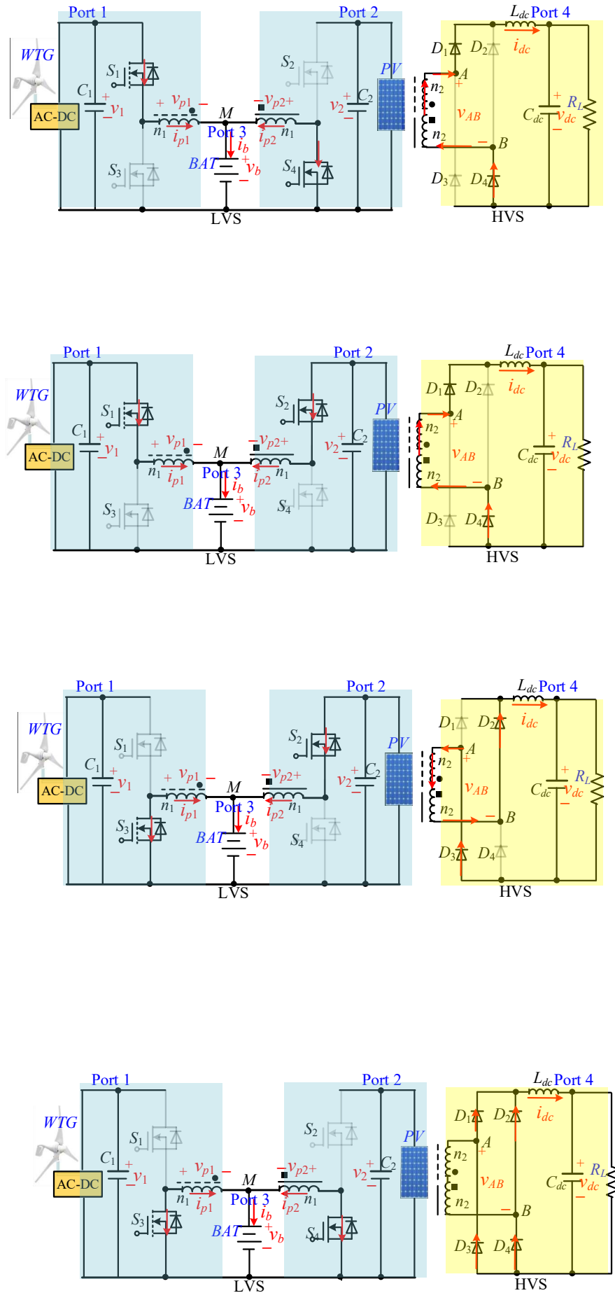
Fig. 4.5 Equivalent circuit of the different operation stage
