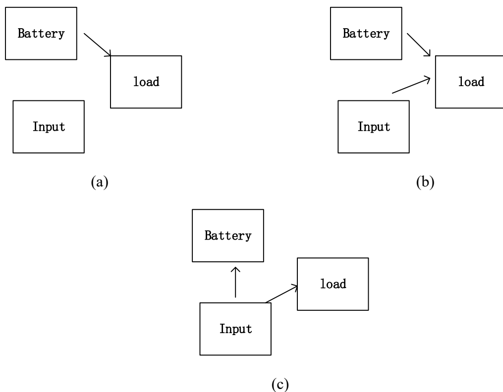
Fig. 2.5 Three port converter working mode: (a)Single input and output; (b)Double input and single-output; (c) Single input and double output.
