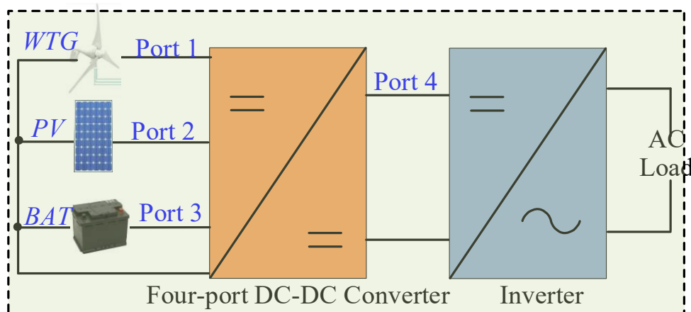
Fig. 4.1 The over viewer of the Four-port DC-DC converter
