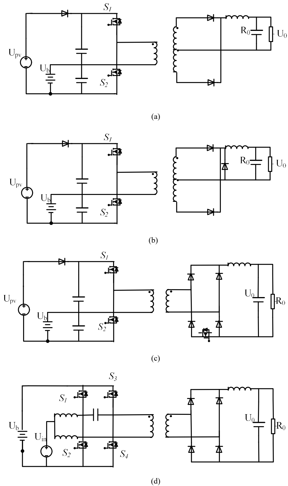
Fig. 1.3 Traditional half-bridge three-port DC converter. (a) originally ...; (b) Secondary side adjustment three-port DC converter; (c) Secondary adjustment three-port DC converter (d) Buck-Boost full-bridge DC converter.
