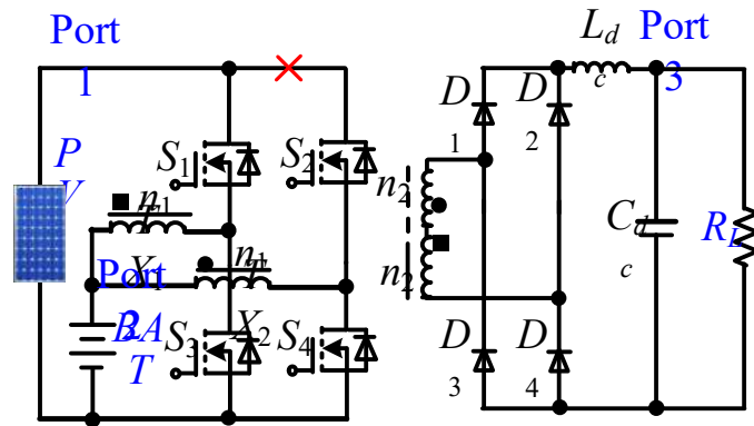
Fig. 4.2 Three-port phase-shift DC-DC converter
