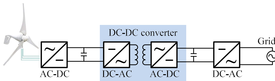
Fig. 1.1 The basic structure of Converter system
