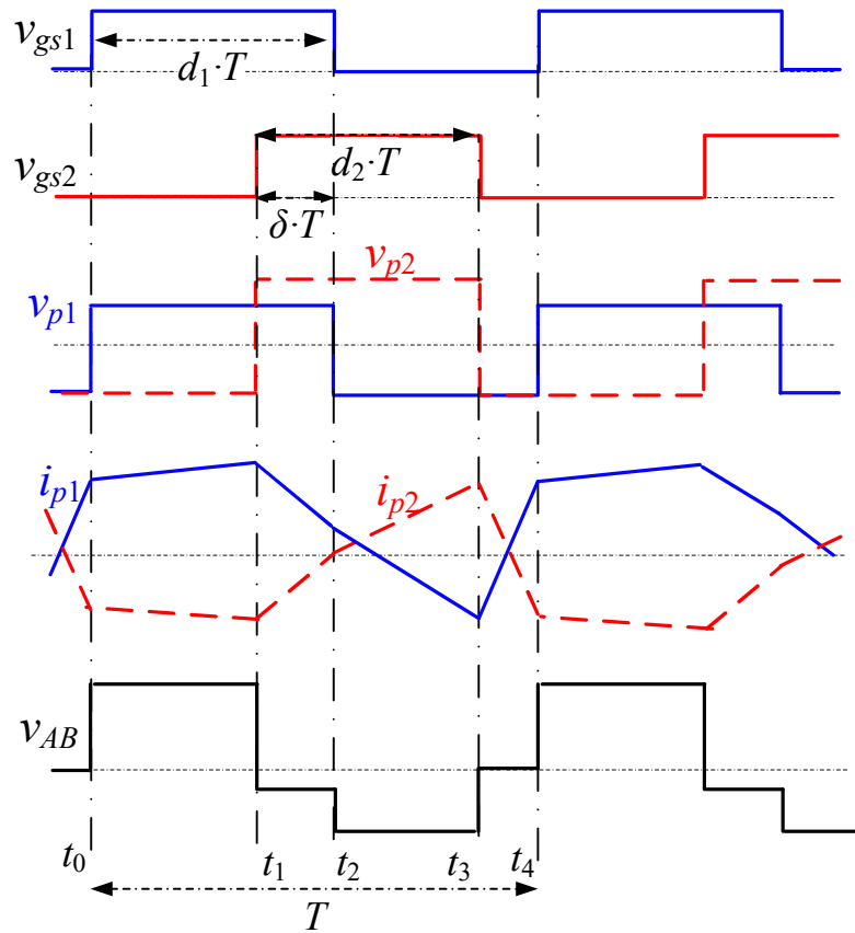
Fig. 4.4 Waveform changing with stage operation
