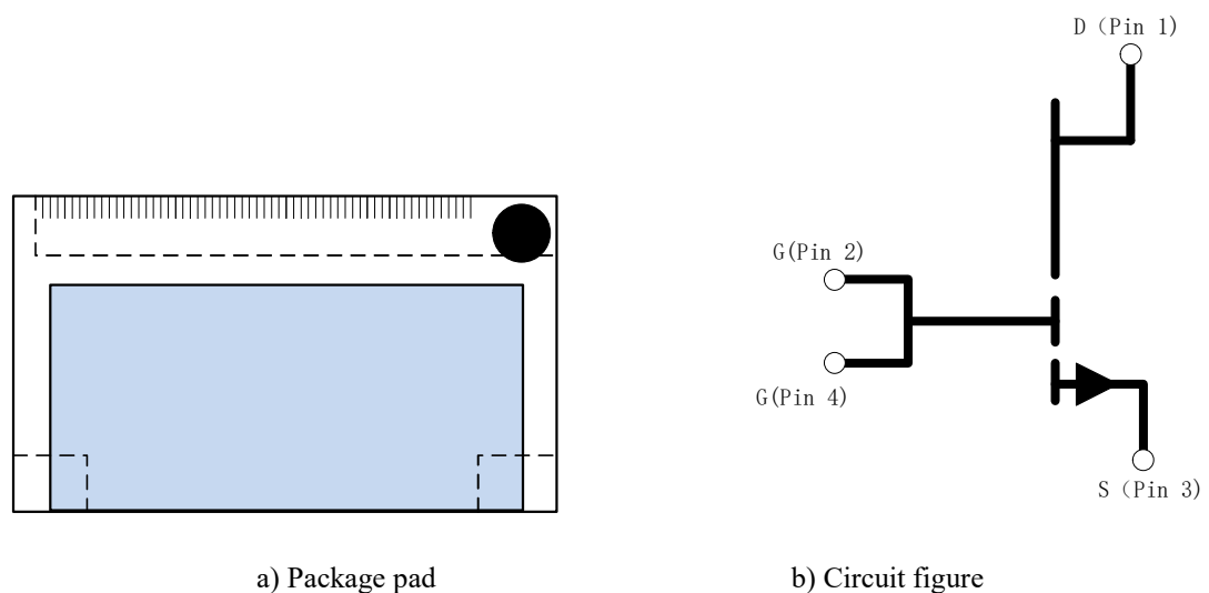
Fig. 3.11 Package outline of GaN package: (a) Package pad; (b) circuit figure.
