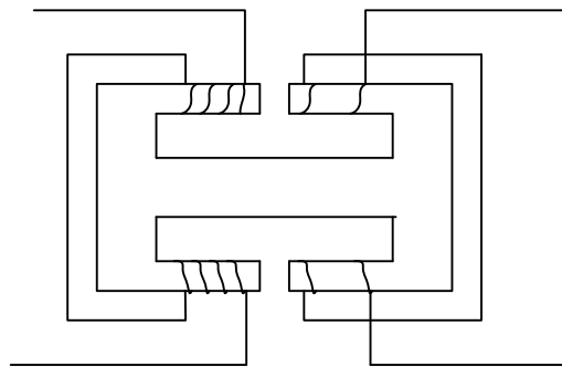
Fig. 3.2 Classical transformer structure
