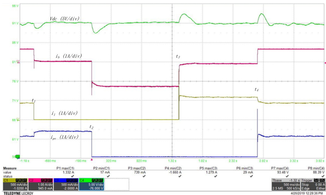
Fig. 5.8 Dynamic processing of switching while regular voltage was 91V
