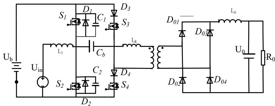
Fig. 2.3 A type of ZVZCS full-bridge Three-port DC converter's topology
