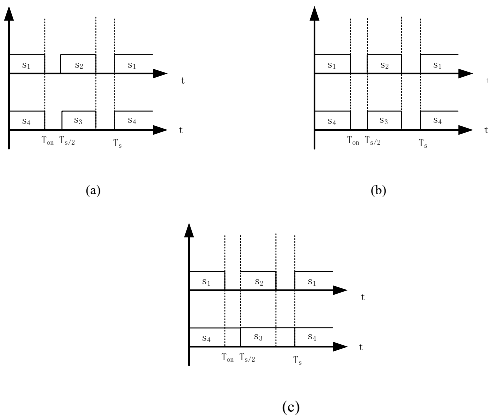
Fig. 2.4 Complementary conduction (a) Bipolar control method (b) finite unipolar control method(c) phase shift control method.
