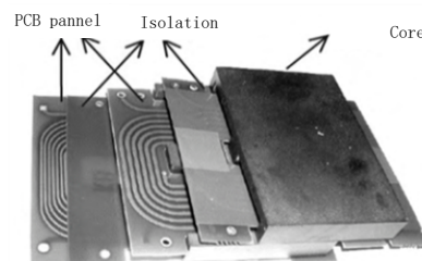
Fig. 3.3 The Panel transformer physical transformer
