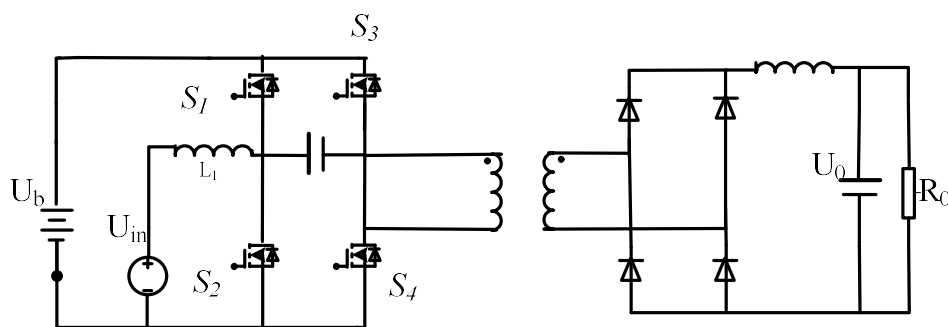
Fig. 2.2 Asymmetric full-bridge three-port DC converter
