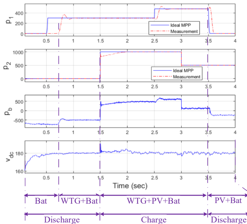
Fig. 5.7 simulation result Converter mode changing
