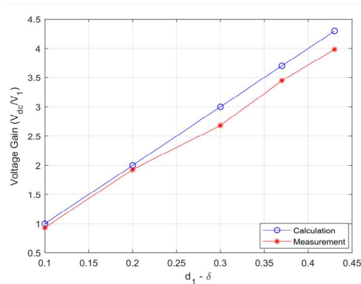
Fig. 5.10 Voltage gain vs. duty cycle
