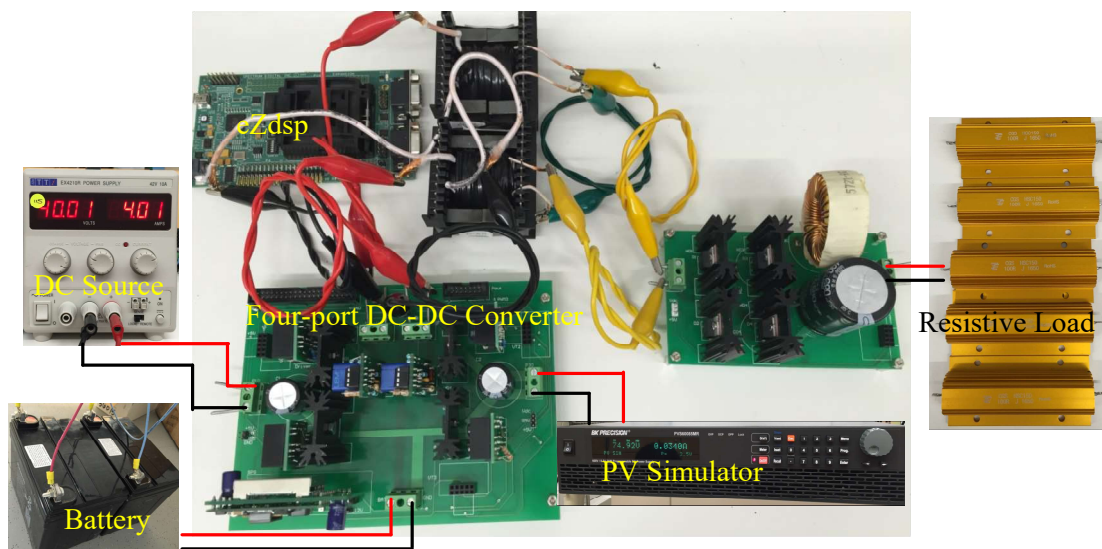
Fig. 5.4 Experiment Setup
