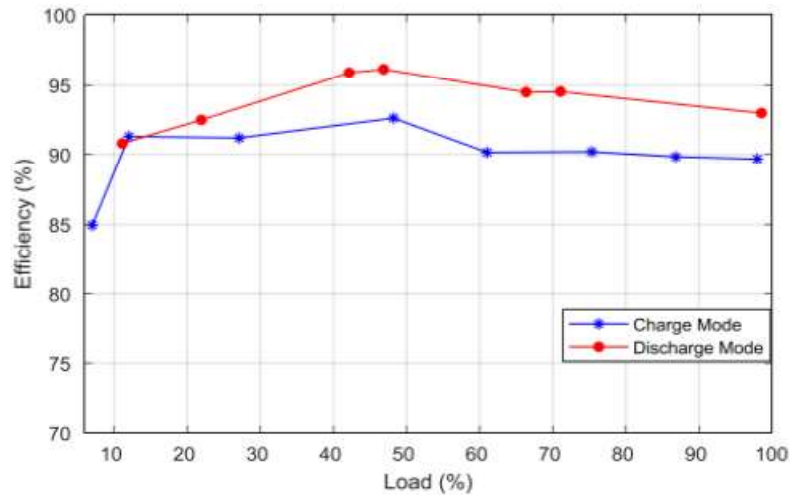
Fig. 5.11 Efficiency measure while charging mode and discharge mode
