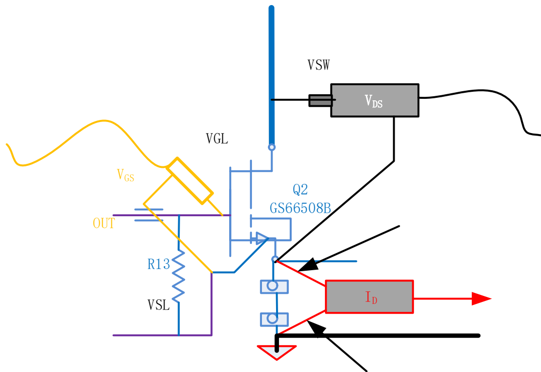
Fig. 3.13 Current shunt connection
