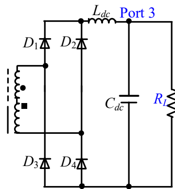
Fig. 3.13 Secondary side of DC converter
