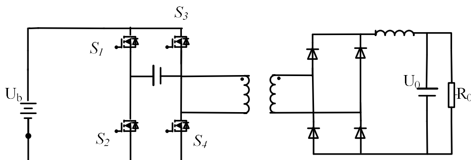
Fig. 2.1 Traditional full-bridge DC converter topology
