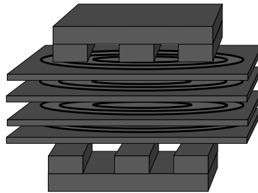
Fig. 3.8 Physical transformer
