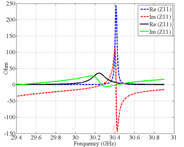
Fig.6 Impact of dielectric lens on the input impedance of the SIW slot antenna obtained by using MoM-PO method (solid-lines show the Z_{11} with lens effects and dash-lines show Z_{11} without lens effects).
