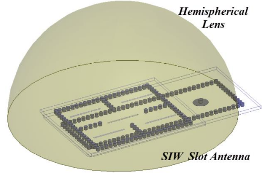
Fig.2 Representation of the entire hemispherical lens antenna.
