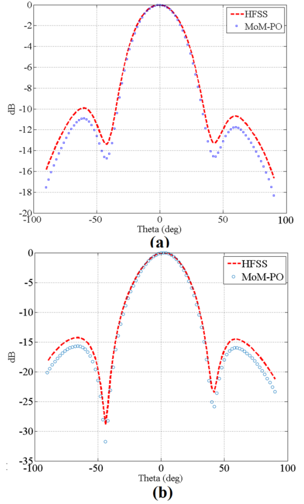
Fig.5 Total field pattern of the ILA computed using the proposed technique and HFSS in (a) \phi = 0 plane, and (b) \phi = 90 plane.
