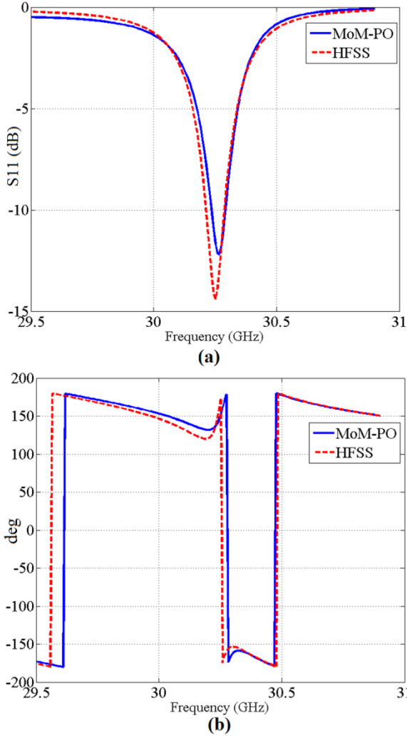
Fig.4 Reflection coefficient of the ILA compared with HFSS, (a) magnitude, and (b) phase.
