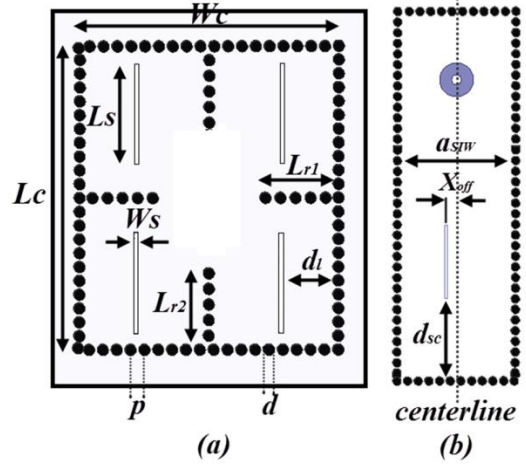
Fig.3 Feeding SIW slot antenna including: (a) cavity and radiating slots placed on top of the substrate, and (b) feeding waveguide and coupling aperture placed on bottom of the substrate.
