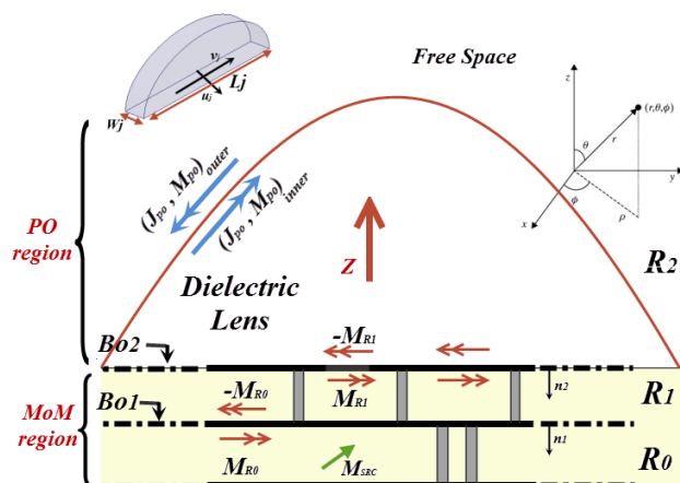
Fig.1 Schematic view of an ILA fed by double layered SIW slot antenna. Also shown is an entire domain basis function shape used to expand the unknown magnetic current on the slot with corresponding parameters.
