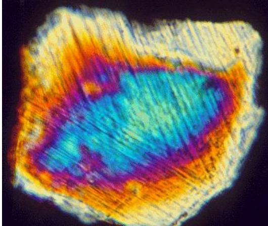
Figure 2: a shocked-quartz grain from the Chesapeake Bay Impact structure. Image from USGS-NASA.
