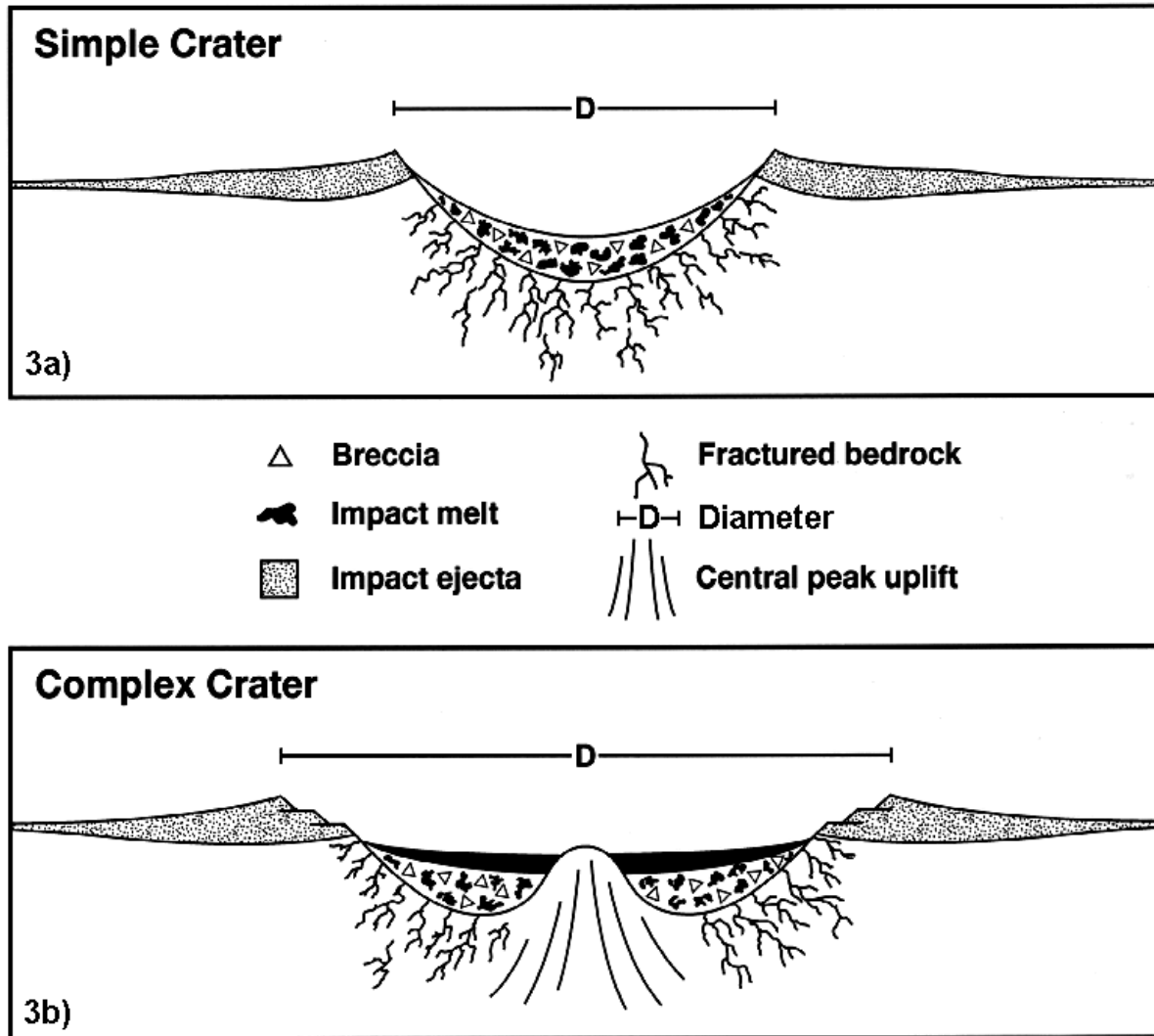
Figure 3: Diagram showing a cross-section of a) a simple crater and b) a complex crater. Modified from http://craters.gsfc.nasa.gov/assests/images/craterstructure.gif
