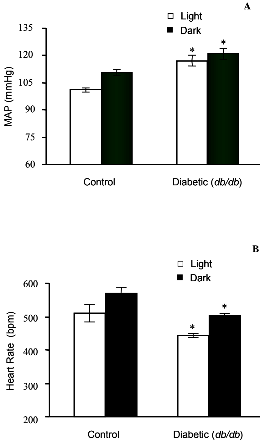
Figure 2: Mean arterial pressure (MAP) and heart rate (HR) in (12-13 weeks old) db/db mice. MAP and HR were recorded in 12-13 weeks old db/db mice and their age matching controls in both light and dark periods (* P < 0.01 control vs. diabetic, n=6 ). Values are expressed as \pm SEM.
