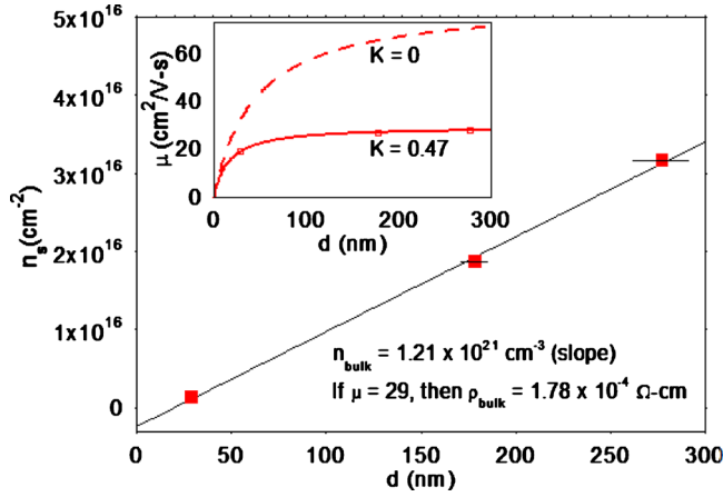
FIG. 1. (Color online) Plots of sheet carrier concentration as a function of layer thickness for samples grown on \text{Al}_2\text{O}_3 . Inset: mobility as a function of thickness. The squares are measured data and the solid line is a fit to these data, with n = 1.2 \times 10^{21} \text{ cm}^{-3} and K = 0.47 . The dashed line is the hypothetical mobility for n = 1.2 \times 10^{21} \text{ cm}^{-3} and K = 0 , or equivalently, N_A \ll N_D .
