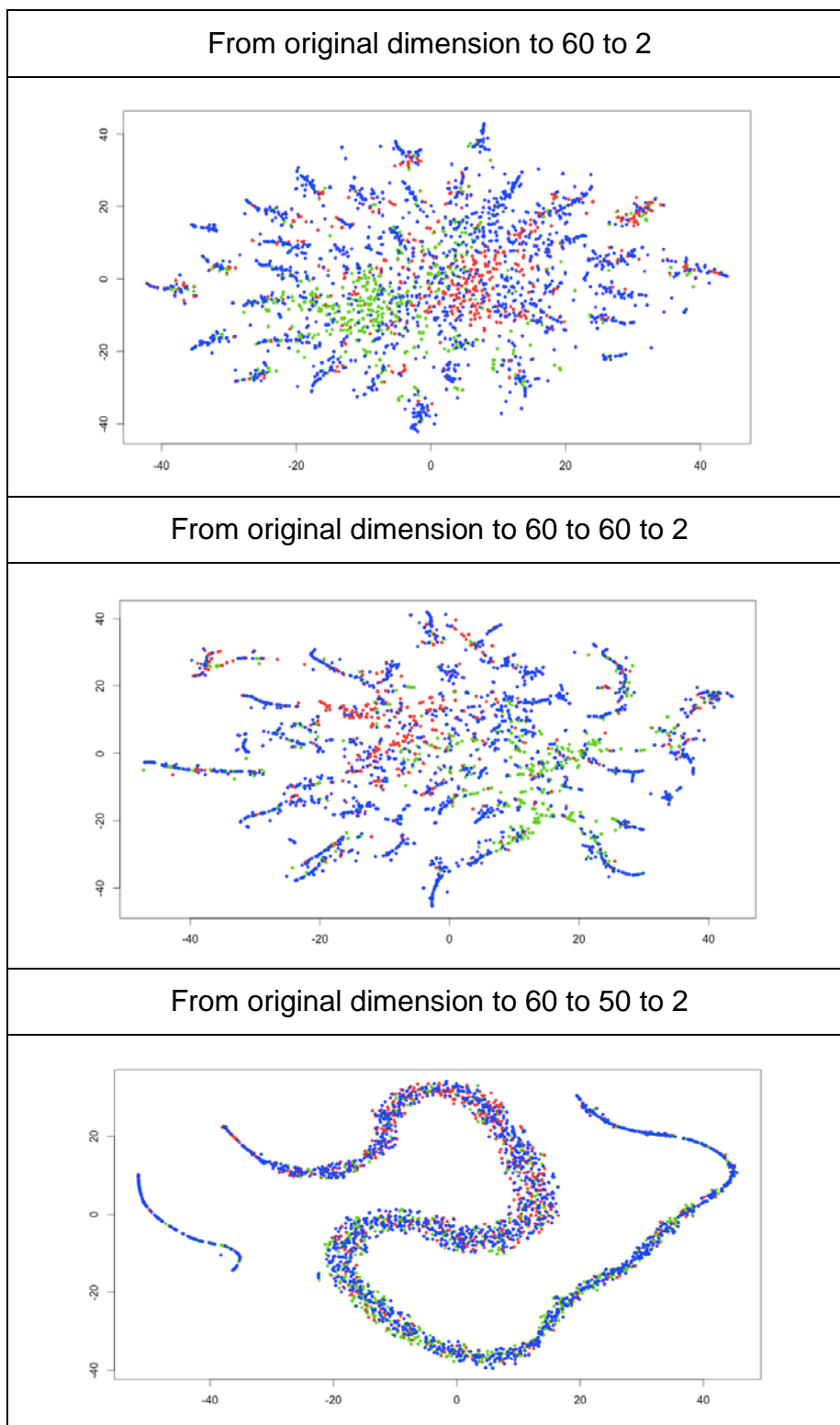
Figure 15. Long path of t-SNE of Splice data using daisy() function
