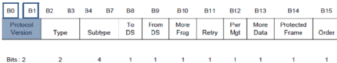
Figure 11. Frame control field [From 6].
