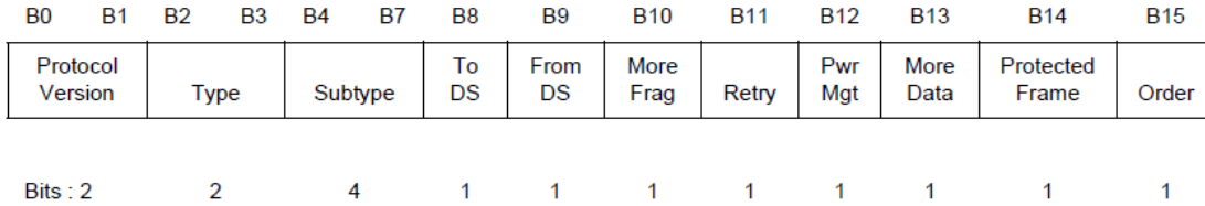
Figure 4. Frame control field [From 6].
