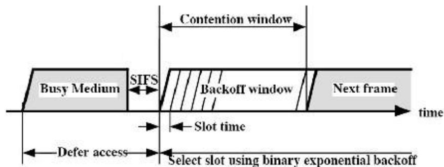
Figure 34. Timing constraints in an 802.11 frame transmission [After 35]
