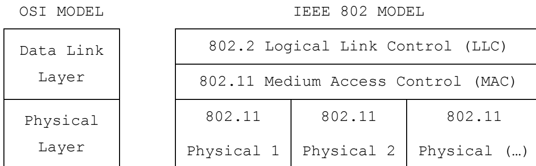
Figure 1. OSI model compared to IEEE 802 protocol architecture.
