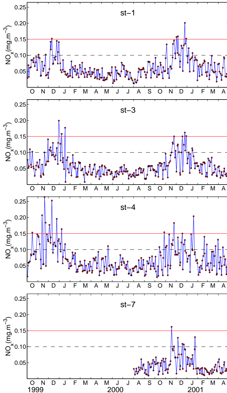
Figure 4. Daily mean \text{NO}_x concentrations ( \text{mg m}^{-3} ) at St-1, St-3, St-4 and St-7 representing four districts. Horizontal dashed line is daily mean second-level criterion, while horizontal solid line is daily mean third-level criterion.
