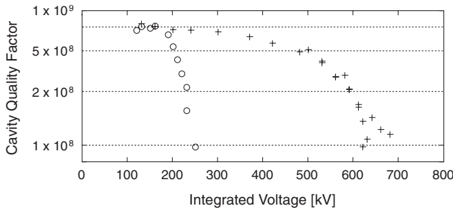
FIG. 12. Cavity Q during testing in September 2009 (circles) and October 2009 (crosses).
