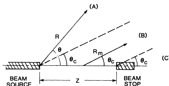
FIG. 1. For a finite path length Z , an observer in regions A or C finds EMP radiation, shown in Fig. 4 and developed in Secs. IIA and IIC. In region B , a Čerenkov field pulse described in Sec. IIB occurs.
