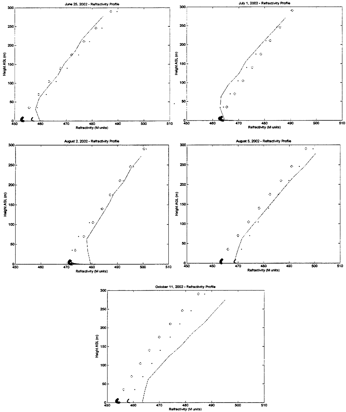
Fig. 6 Profiles from the Nellis AFB observation site display the M unit refractivity for sounding data (solid line), 6-km model domain data (open circles) and 2-km domain data (dots) from 0830 UTC on each test day. Profiles extend from the surface to 300 meters above ground level (AGL). Monin-Obukhov values are visible below 10 meters in the model curves and below 2 meters in the sounding curves. A change in the sign of dM/dz from negative to positive above the surface in the June 25, July 1 and August 2 observations indicates ducting. Overall, 2-km grid profiles are slightly closer to observation profiles than 6-km grid profiles, particularly near the surface.
