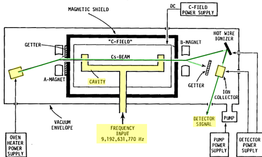
Cesium Atomic Beam Oscillator
