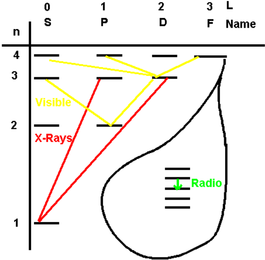
Energy Levels Complex Atom
