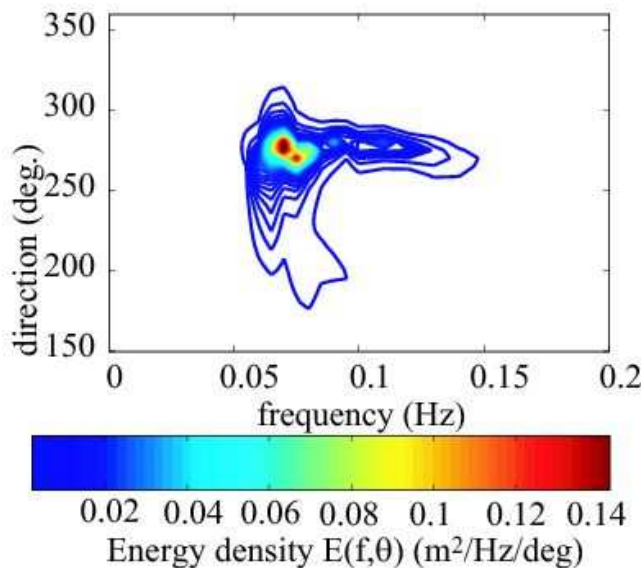
Figure 10. Directional wave spectrum at Torrey Pines Outer Buoy at 15:00 UTC on 30 November 2003.
