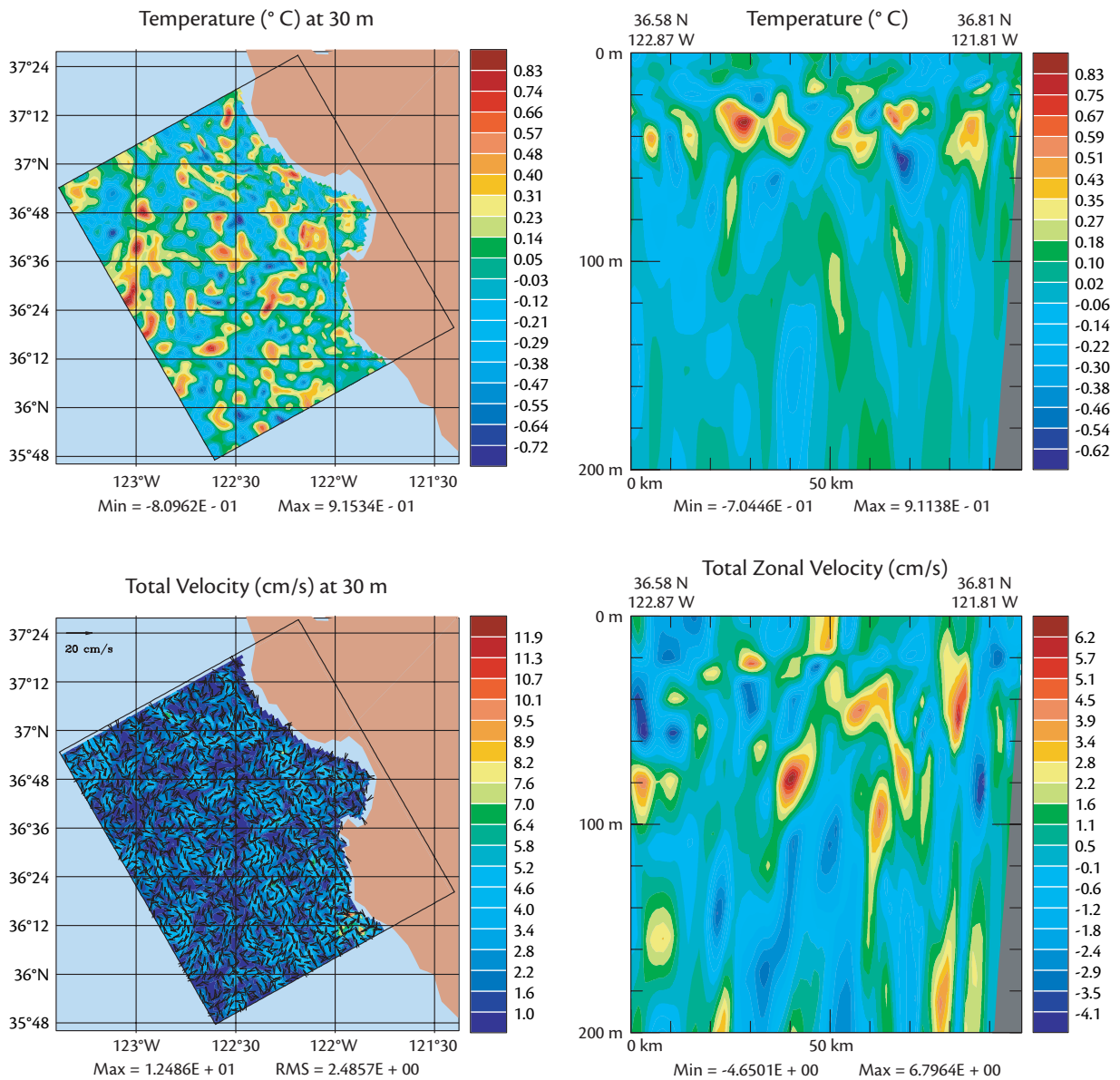
Figure 2. Illustration of the effects of adding random forcings, correlated in time and space, to a PE model. Shown are differences between a deterministic and stochastic PE model simulation over the Monterey Bay and California Current System region, after one day of integration. Differences in horizontal maps of T and \|u_h\| are shown at 30-m depth (top and bottom left) and in cross sections (from offshore to the coast in Monterey Bay) of T and u , from 0–200 m depth. The amplitudes of the random forcings were set to a fraction (25 percent) of the average geostrophic balance at each depth ( \|geostrophy(z)\| ), with a half-day decorrelation in time and one-to-two grid point correlation in space. Geostrophy is not always the sole component of the dominant PE balance in the region. Future random forcing models will for example include impacts of atmospheric forcing in the balance.
