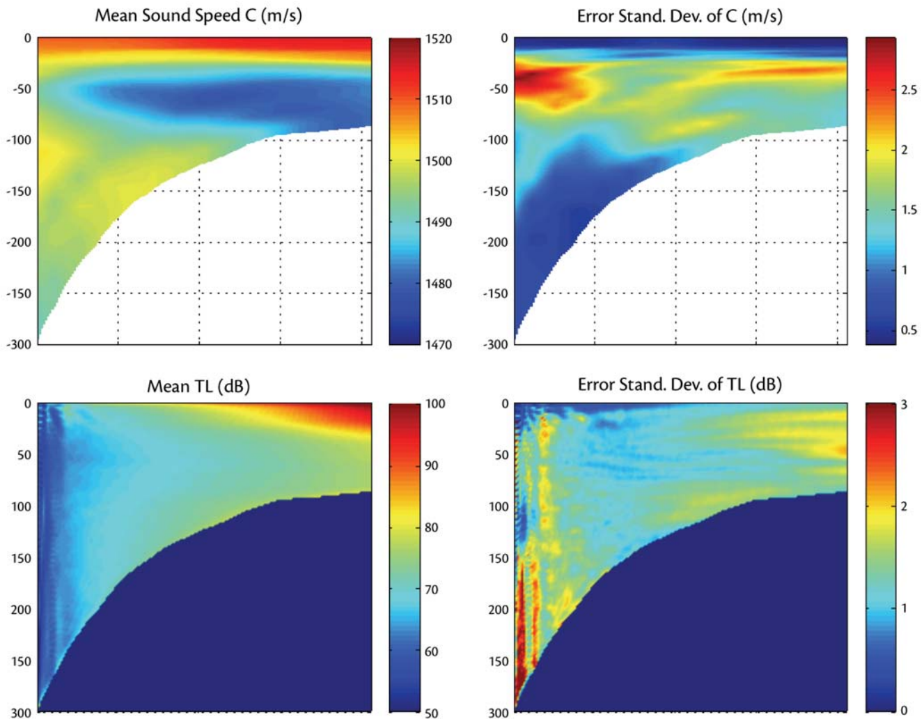
Figure 6. Cross sections on July 26, 1996 in the mean and error standard deviations Error Subspace Statistical Estimation (ESSE) estimates of the sound-speed (top) and broadband TL (bottom) along the main acoustic section (western section of the PRIMER experiment). Note that if we also model uncertainties in the bottom attenuation coefficient (not shown), we find that the mean TL remains similar, but the TL error standard deviation increases substantially in the surface mixed layer above the shelf. This is a result of the uncertain attenuation at each acoustic bottom bounce and shows the importance of seabed uncertainties in acoustic predictions.
