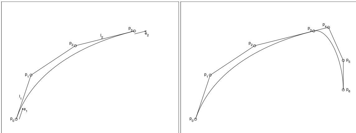
Figure 4: Bezier Segments Showing Notation. (a) One Segment Bezier, (b) Two Segment Bezier
