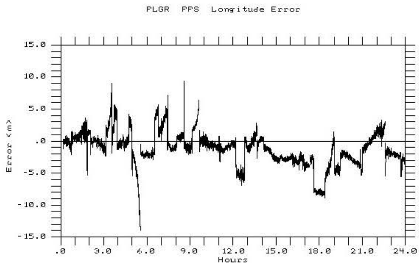
Figure 3: PLGR PPS Error While Static
