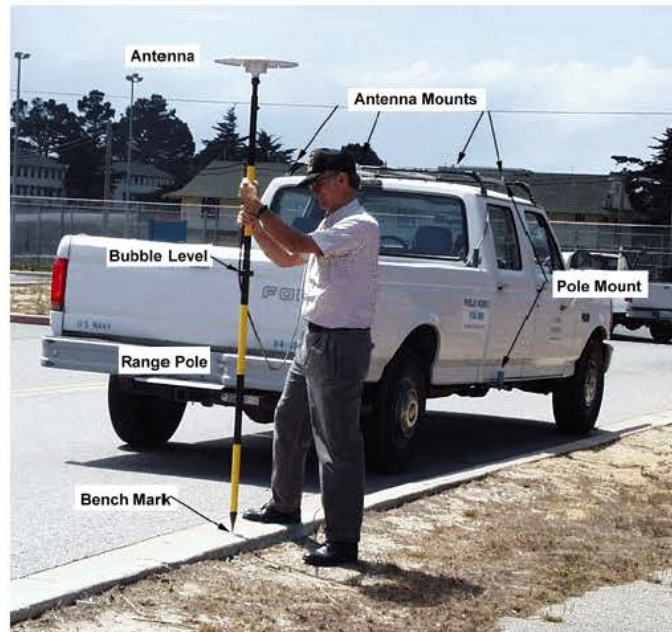
Figure 9: Vehicle Used for Data Acquisition
