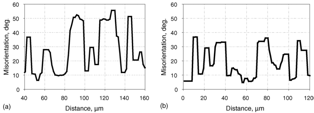
Fig. 2. Point-to-origin disorientation profiles for ECAP aluminum processed by route B C : (a) the 90° sample, four passes and (b) the 135° sample, eight passes.
