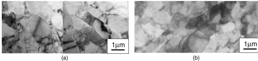
Fig. 4. TEM images of ECAP (route B C ) aluminum: (a) 90° sample, four passes and (b) 135° sample, eight passes.
