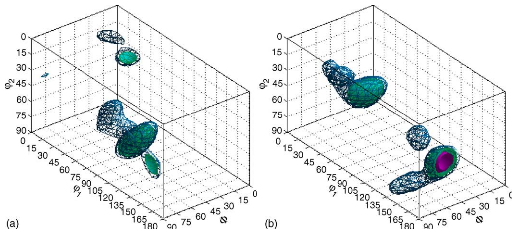
Fig. 3. 3D ODFs for ECAP aluminum processed by route B C : (a) the 90° sample, four passes and (b) the 135° sample, eight passes. Iso-surfaces correspond to 1/8, 1/4 and 1/2 of the maximum intensity in each case.
