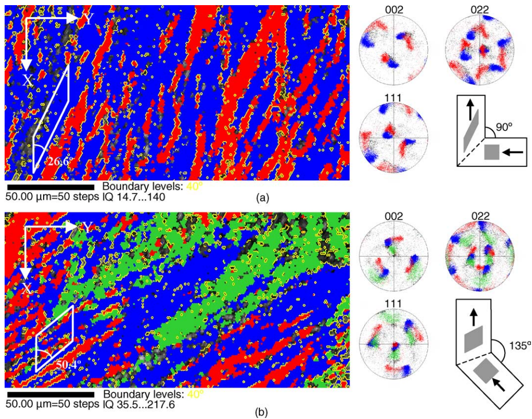
Fig. 1. OIM maps and pole figures for aluminum after (a) 90° sample, four passes and (b) 135° sample, eight passes. Gray-scale maps and pole figures were highlighted by different colors corresponding to characteristic orientations in the textures. The insets with the pole figures indicate the orientation of the die sets relative to the sample coordinates.
