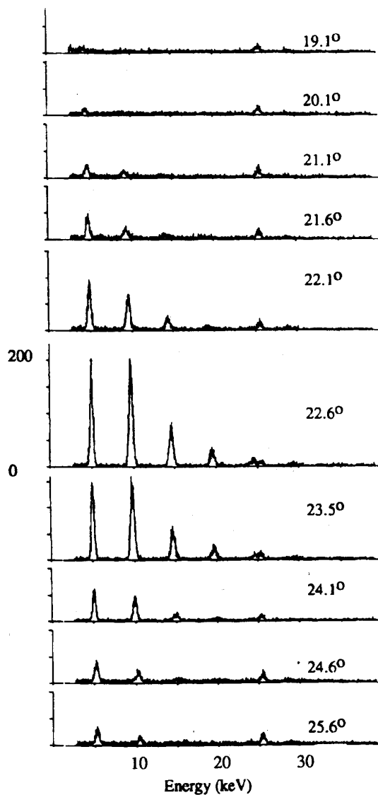
Figure 3. PXR spectra from the (002) plane of mosaic graphite, observed with the detector fixed at 45^\circ and the crystal oriented at the indicated Bragg angles. The tin fluorescence line at 25.2 keV serves as an energy and beam intensity calibration peak.
