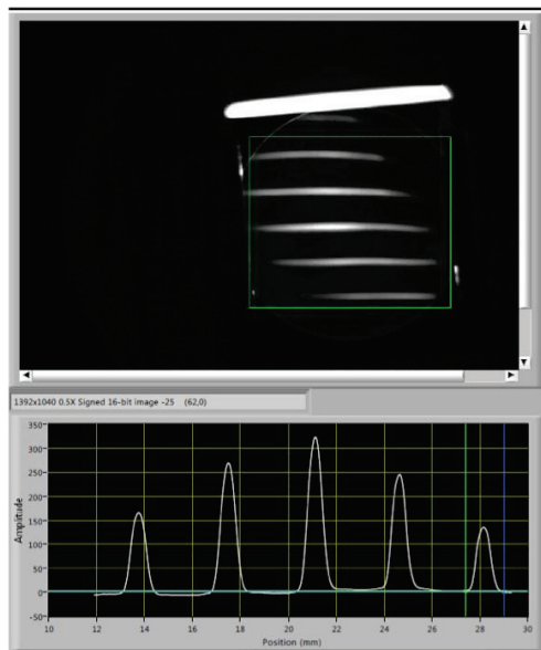
Figure 6: Electron beam image from diagnostic station 2 showing beamlets (upper panel). The lower panel shows the projected intensity along the axis (white line). Each beamlet is windowed individually and combined to obtain the final emittance value.
