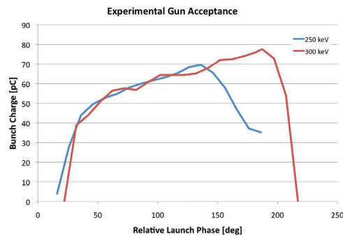
Figure 5: Cavity acceptance curves for two beam energies: 250 keV and 300 keV.
