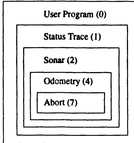
Figure 9: Interrupt Hierarchy
