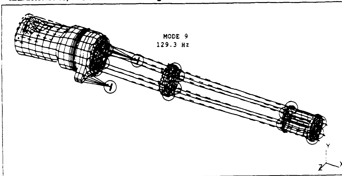
Figure 4.15. Isometric view of MODE 9.
