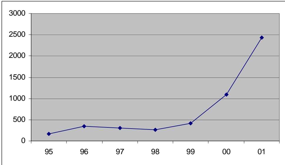
Figure 2. Vulnerabilities Reported to CERT/CC.
