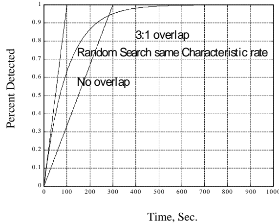
Figure 7. Comparison of random search with overlapping direct search and non-overlapping direct search showing that 3:1 overlap may be worse than random search. [Results are for assumed uniformly distributed targets with independently random search paths with no obstacles, no other searchers, and no boundaries].
