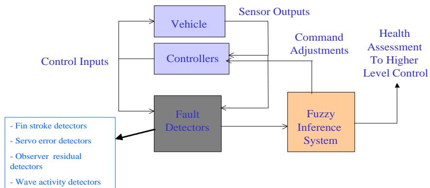
Figure 2 Fault Detection Architecture Including Fuzzy Inference System for Resolution of Fault State
