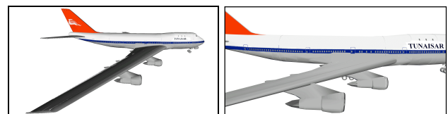
Figure 3. Savage model of 747 aircraft seen from 25M with FOV 1.57 (90°) and then less-distorted FOV 0.7853 (45°)
