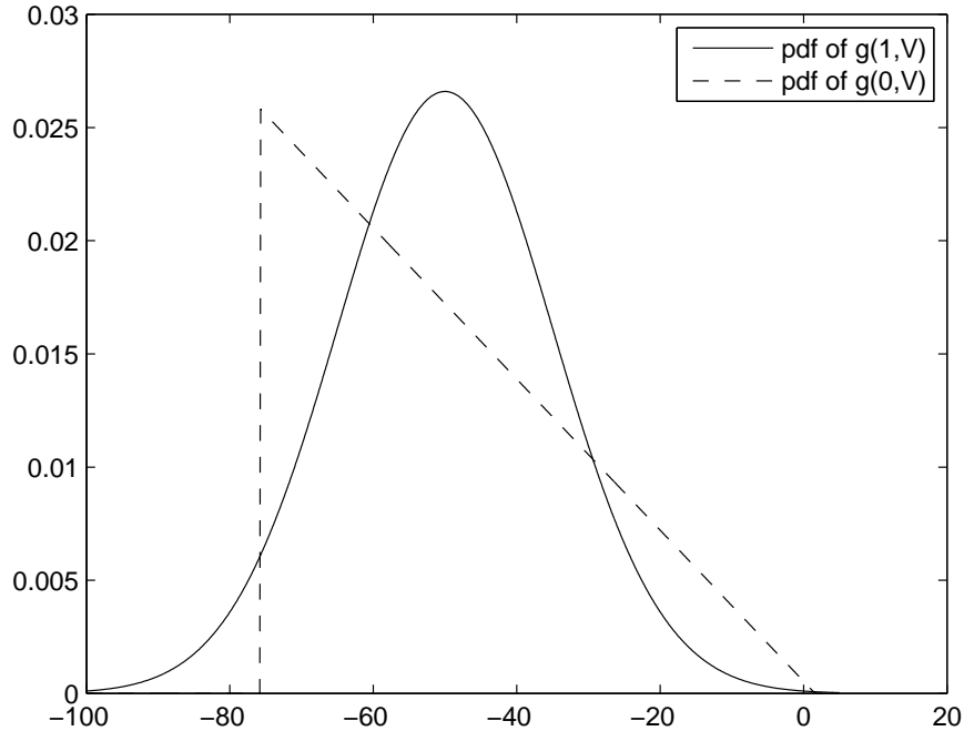
Figure 1: Example 1: Probability density functions (pdf) of g(1, \mathbf{V}) and g(0, \mathbf{V}) .
