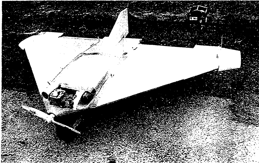
Fig 2.8 - Exdrone UAV
