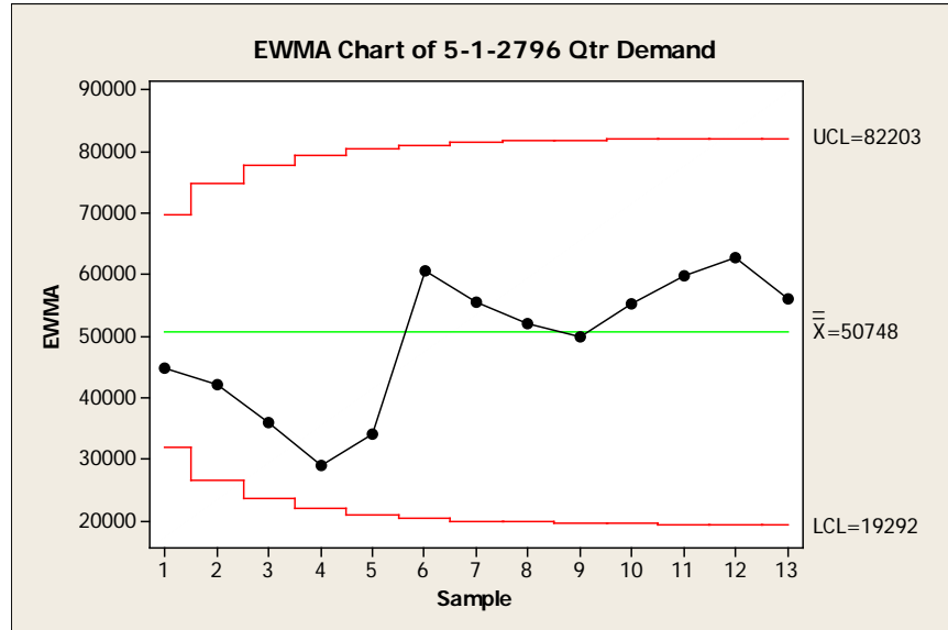
Figure 18. EWMA Chart for 5-1-2796
