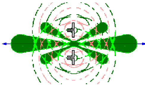
Figure 5. Two Elements Fed with the Same Phase
