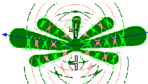
Figure 6. Two Elements Fed with Different Phases
