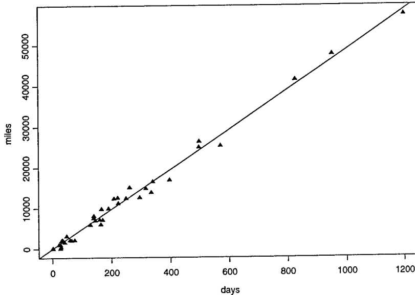
Figure 2.1: Traction Motor Data with Regression Line. Triangles represent the number of days and miles until a failure occurred.
