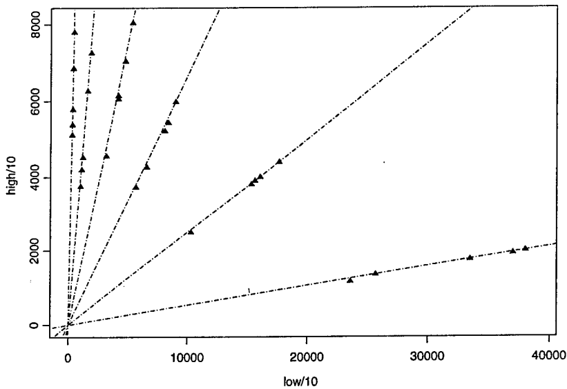
Figure 2.3: Metal Data with Approximate Linear Usage Paths. Each triangle represents the number of low-load and high-load cycles until a failure occurred, scaled by a factor of 1/10.
