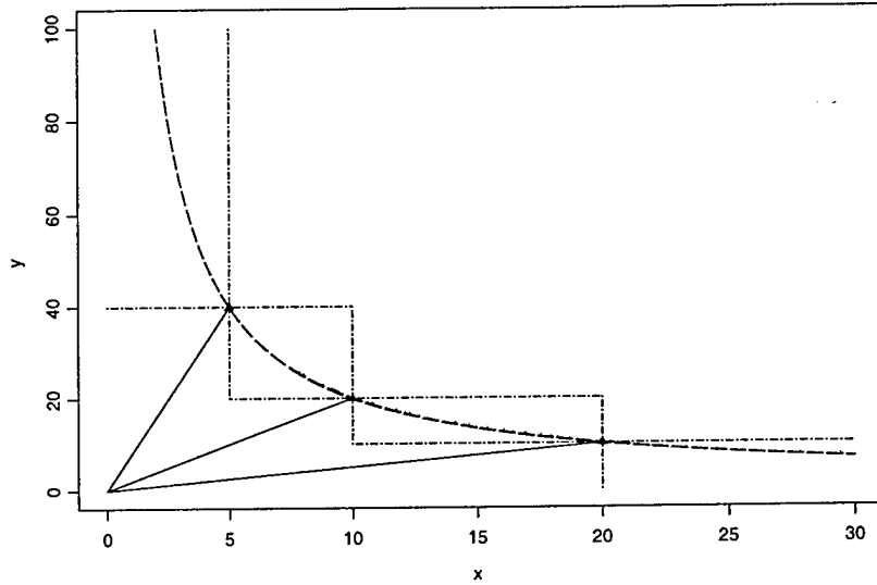
Figure 4.2: Extension of Estimated Optimal Policy. The solid lines represent the failure replacement region for the policy with replacement time vector (20, 10, 5) . The dashed lines represent bounds for a non-increasing function serving as a policy boundary under the lower set restriction. The smooth curve represents the boundary of one possible extension of the policy based on the linear paths of slope 0.5, 2, and 8.
