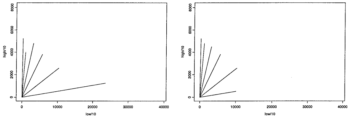
Figure 2.4: Composite Policies for the Metal Data. The solid lines on left side of the figure represent the failure replacement region for the policy with replacement time vector (23580, 10300, 5700, 3200, 1000, 275). The right side of the figure depicts the failure replacement region for the policy with replacement time vector (10000, 10300, 5700, 3200, 1200, 275).
