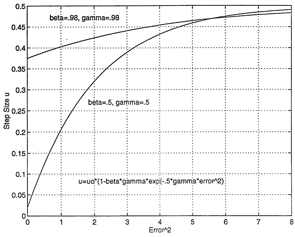
Figure 6a Variation of u with Error 2 for u_0 = 0.05
