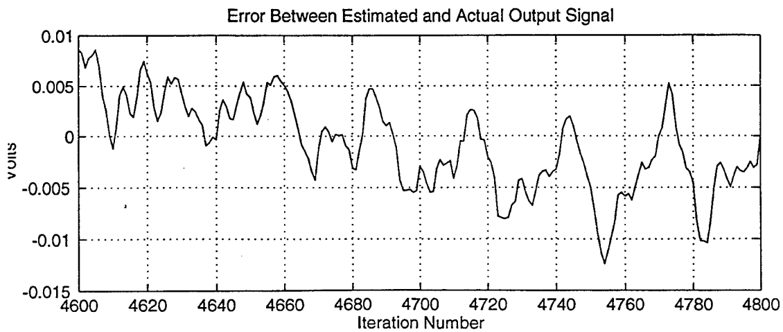
Figure 14d Results Using an IIR Filter on a Nondispersive System (Aluminum Bar)
