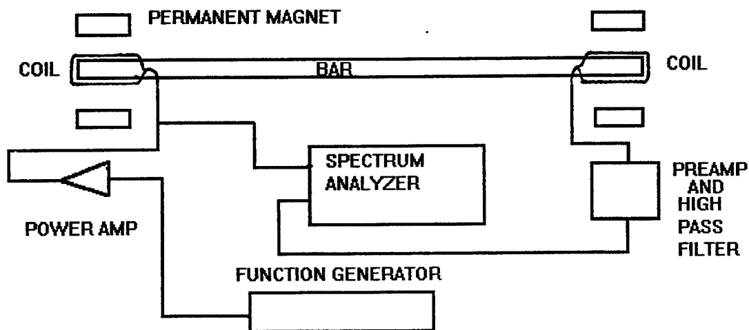
Figure 3a Electrodynamic Transduction
