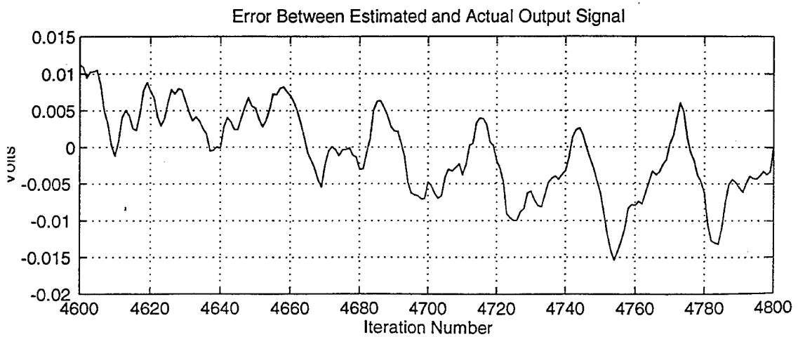
Figure 14c Results Using a FIR Filter on a Nondispersive System (Aluminum Bar)
