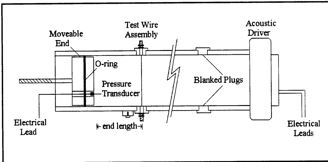
Figure 6. Acoustic Chamber and Accessories
