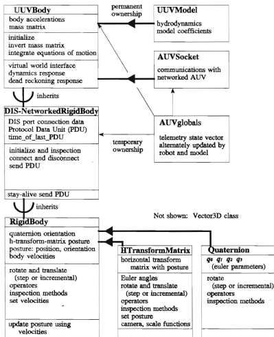
Figure 6.7. General real-time DIS-networked hydrodynamics model class hierarchy.
