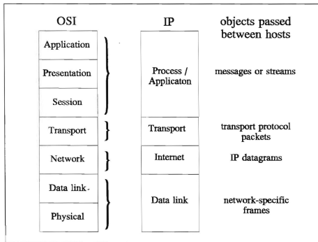
Figure 7.1 Correspondence between OSI and IP protocol layer models, and objects passed between corresponding layers on separate hosts.
