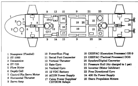
Figure 4.3. NPS AUV II internal components layout (Torsiello 94).
