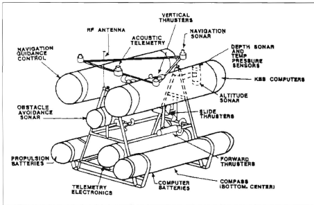
Figure 2.4. Marine Systems Engineering Laboratory (MSEL) Experimental Autonomous Vehicle EAVE II equipment layout (Blidberg 90).
