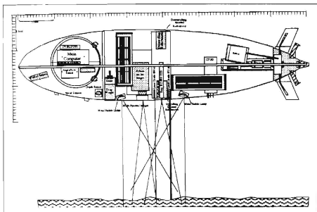
Figure 2.5. Florida Atlantic University Ocean Voyager II (Smith 94).
