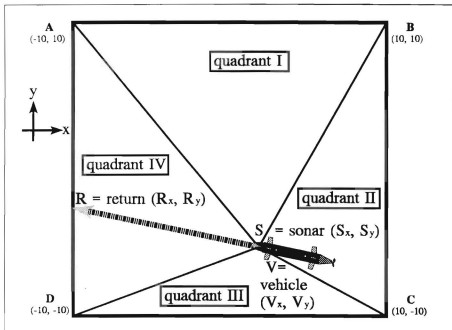
Figure 8.3. NPS AUV test tank geometry.
