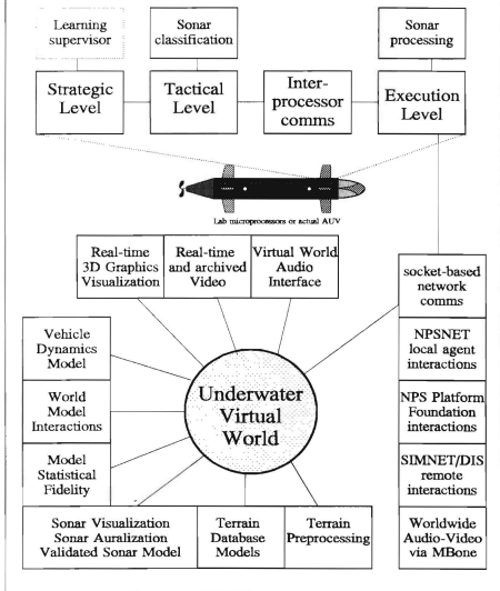
Figure 3.1. NPS AUV underwater virtual world software architecture.
