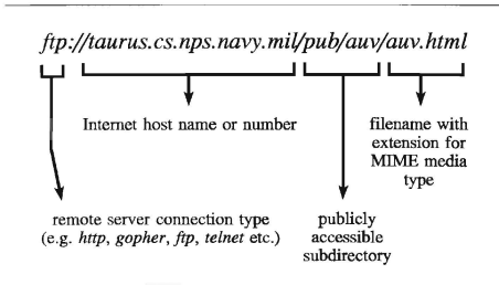
Figure 7.4. Example Universal Resource Locator (URL) components.
