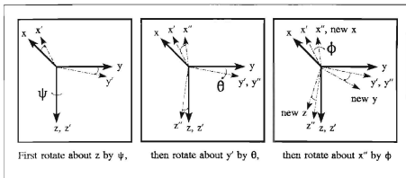
Figure 6.4. Intermediate rotation axes for Euler angle rotations from world coordinate frame to body coordinate frame, adapted from (IEEE 94a).
