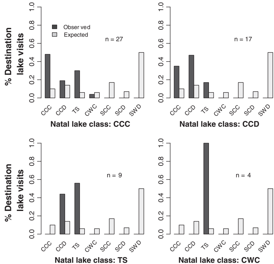
FIGURE 5 The proportion of juvenile loons visiting different lake types relative to their own natal lake class. Juvenile loons originating from Cool-Complex-Clear (CCC) lakes, Cool-Complex-Dark (CCD) lakes and Two-Story (TS) lakes visited their own lake classes in greater proportions than would be expected given the background distribution of lake classes (CCC: \chi^2 = 81.93 , df = 6 , p < 0.0001 ; CCD: \chi^2 = 39.81 , df = 6 , p < 0.0001 ; TS: \chi^2 = 49.96 , df = 6 , p < 0.0001 ). Other designations include Complex-Warm-Clear (CWC) lakes, Simple-Cool-Clear (SCC) lakes, Simple-Cool-Dark (SCD) lakes, and Simple-Warm-Dark (SWD) lakes
