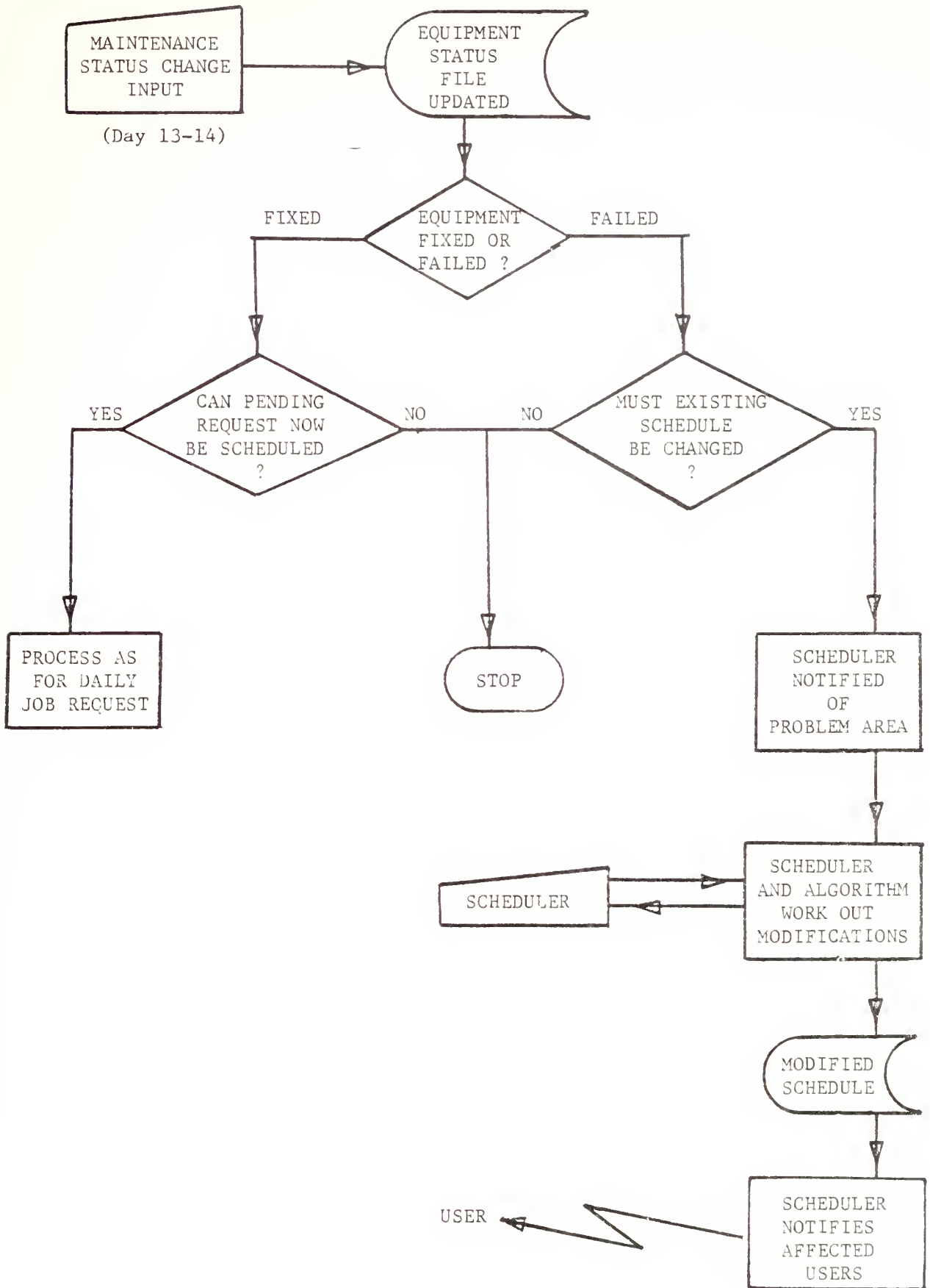
Figure 4. Flowchart for Maintenance Status Change
