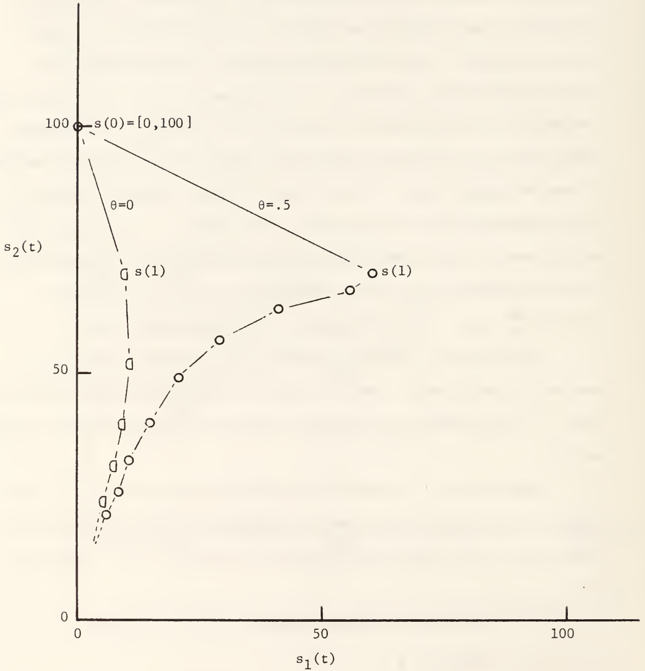
Figure II.4: Plot of s(t) for example 7 using \theta=0.5 and \theta=0 , s(0)=[0,100]
