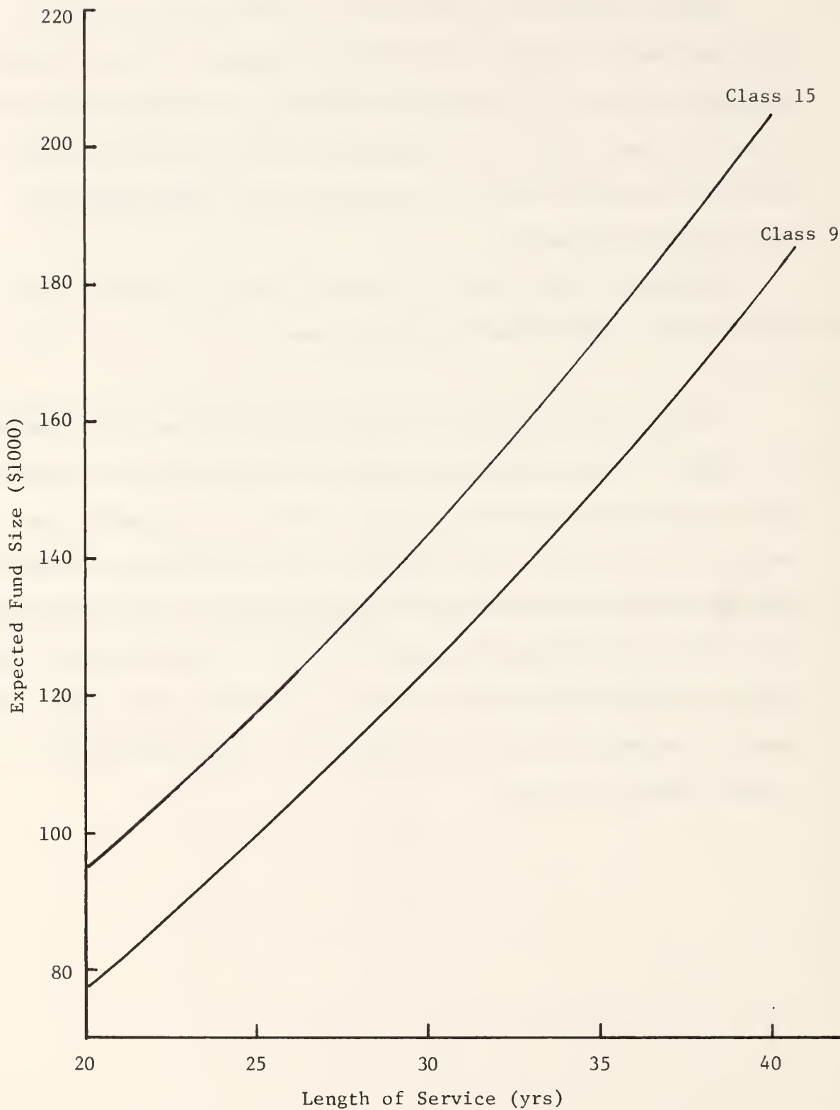
Figure II.8: Expected Retirement Fund Size for Faculty Example.
