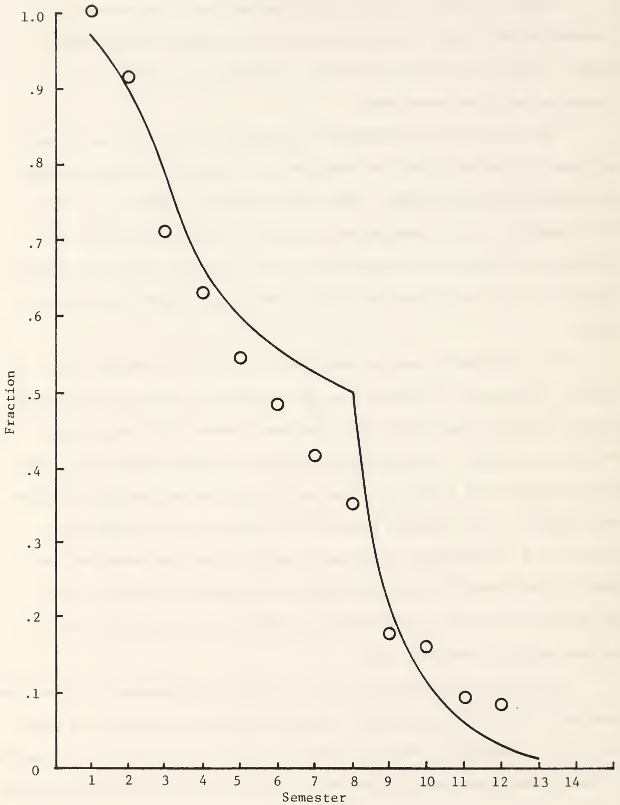
Figure II.12: Fraction in Attendance; 5 Class Model.
