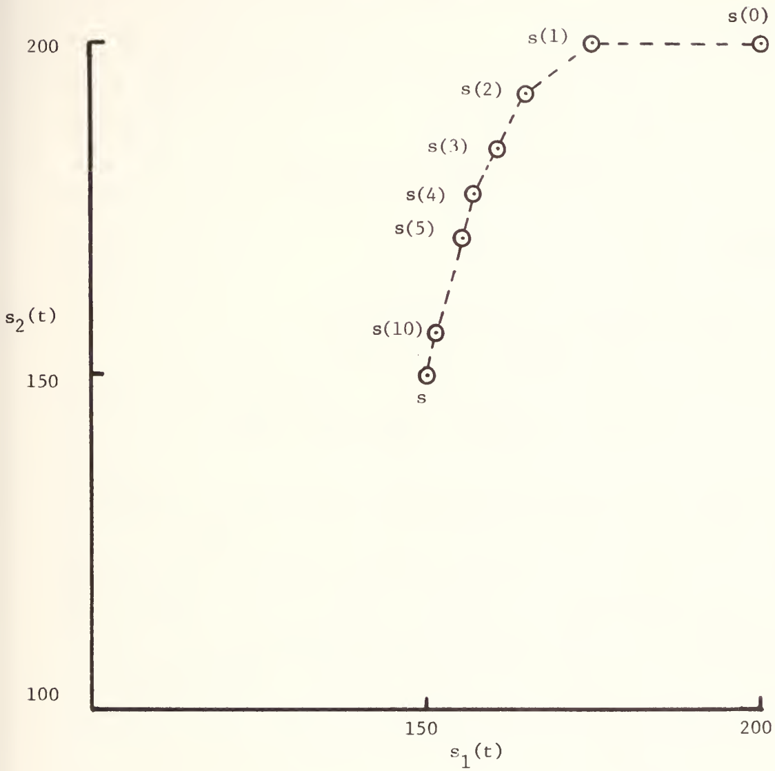
Figure II.5: Plot of S(t) for Example 8, a decreasing organization
