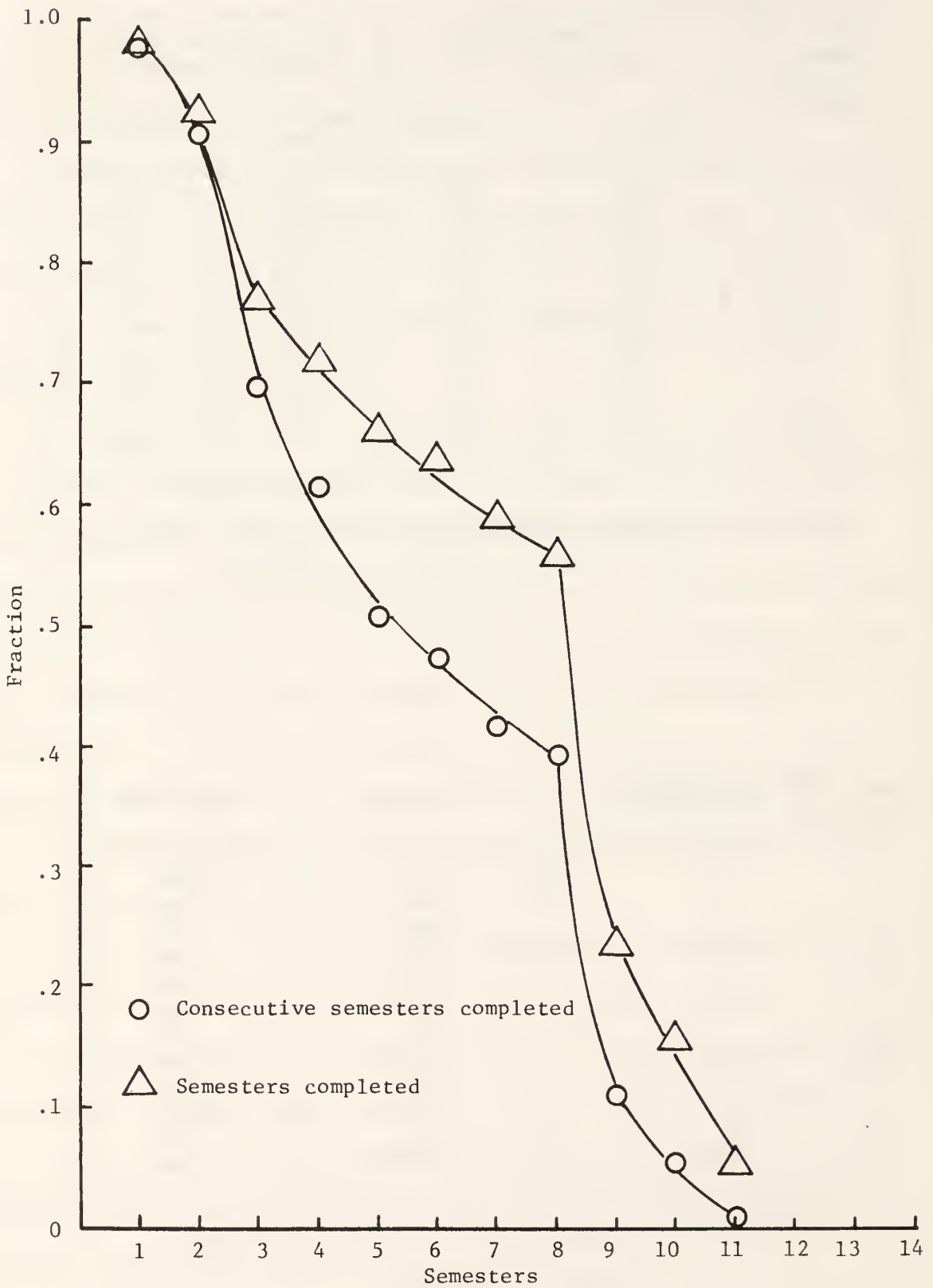
Figure II.10: Fraction with Consecutive Attendance and Elapsed Time (1960 Data).
