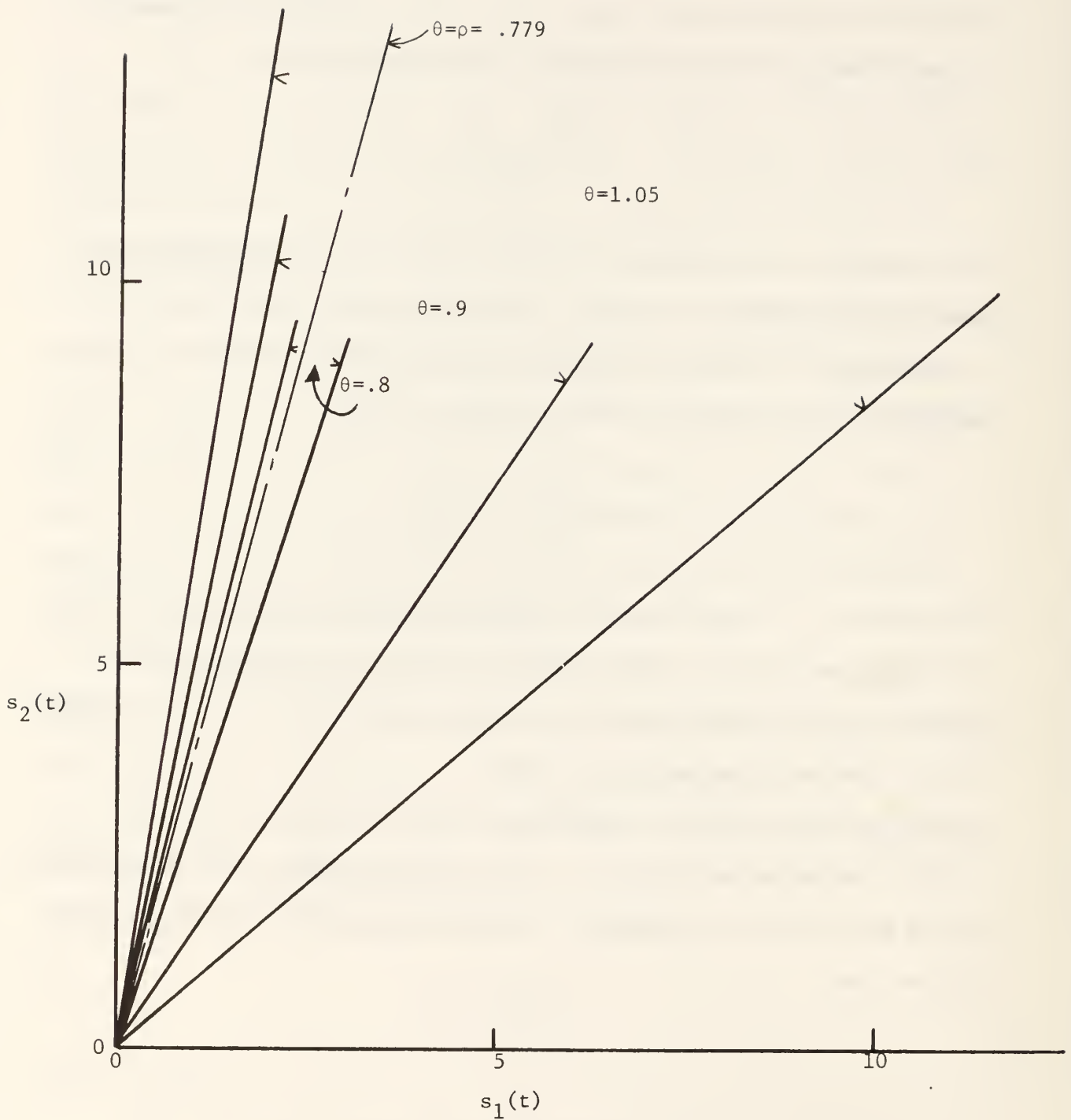
Figure II.6: Sets of Feasible Initial Vectors for various Geometric Growth rates
