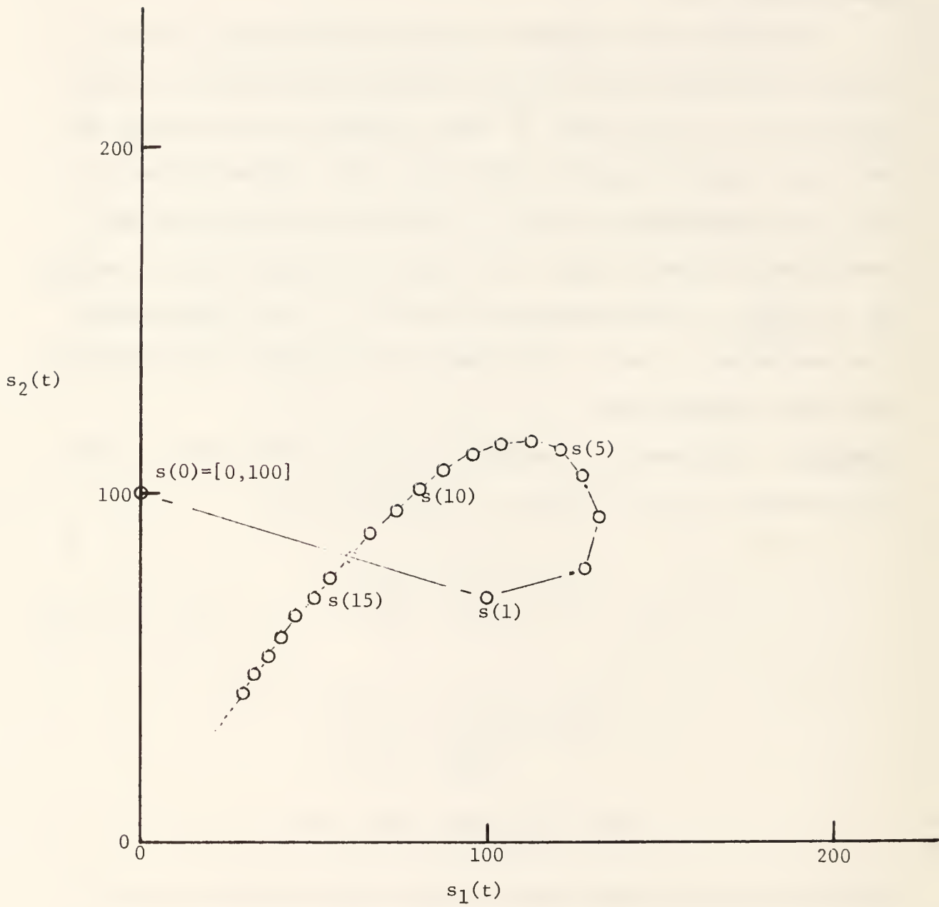
Figure II.3: Plot of s(t) for Example 6 using \theta=.9 , s(0)=[0,100]
