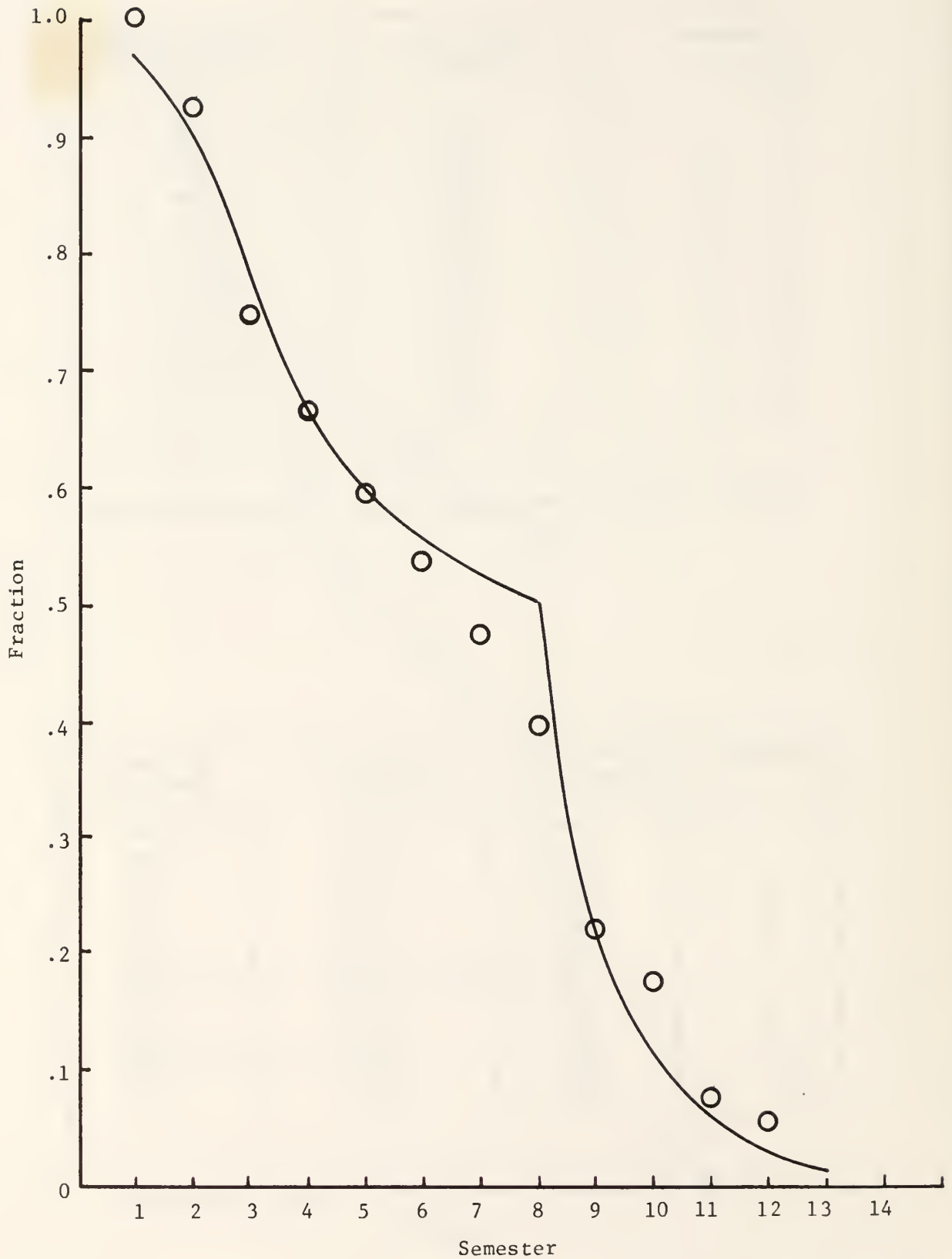
Figure II.11: Fraction in Attendance; 4 Class Model.
