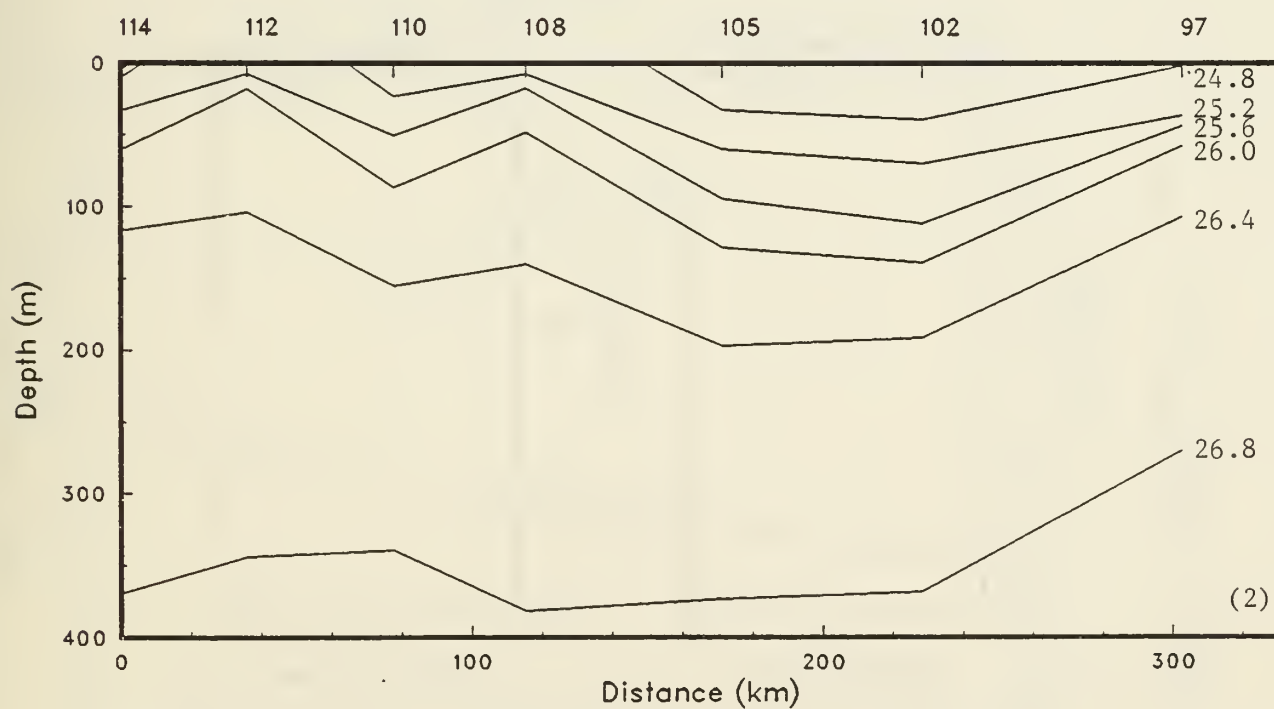
Figure 30(a): Isopleths of (1) temperature and salinity and (2) \sigma_t from the CTD's (OPTOMA16, Leg A).
