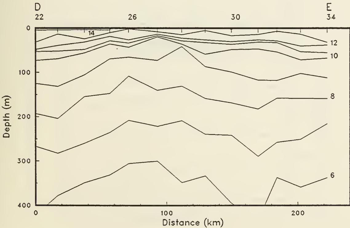
Figure 18 (a)-(b): Along-track isotherms. Tick marks along the upper horizontal axis show station positions. Some station numbers are given. Dashed lines are used if the cast was too shallow (OPTOMA16, Leg MII).
