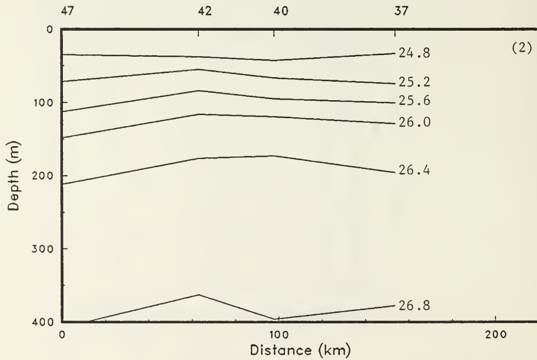
Figure 19(a): Isopleths of (1) temperature and salinity and (2) sigma-t from the CTD's (OPTOMA16, Leg MII).
