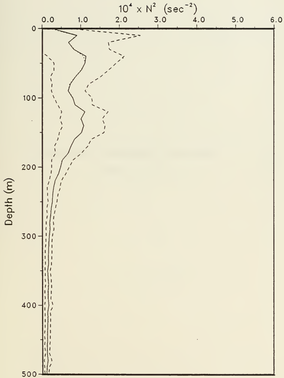
Figure 12: Mean N^2 profile (—), with \overline{+} and \overline{-} the standard deviation (---). The N^2 profile from \overline{T(z)} and \overline{S(z)} is also shown (...) (OPTOMA16, Leg MI).
