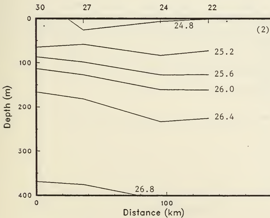
Figure 8(a): Isopleths of (1) temperature and salinity and (2) \sigma_t from the CTD's (OPTOMA16, Leg MI).
