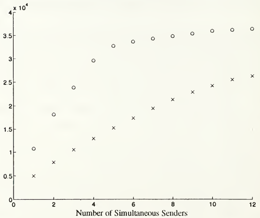
* = Tree Cost for Receive Tree Rooted at Selected Center o = Tree Cost for Send Tree Rooted at Selected Center + = Tree Cost for Receive Tree Rooted at Least Cost Center x = Tree Cost for Send Tree Rooted at Least Cost Center
