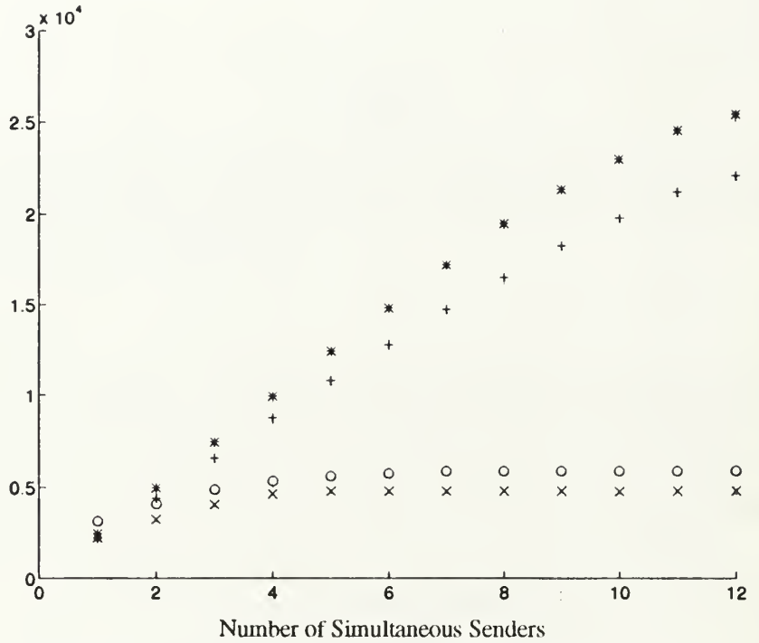
x = Center-Specific Tree, o = Source-Specific Tree Figure 10. Tree Cost vs. Simultaneous Senders on Final Interaction
