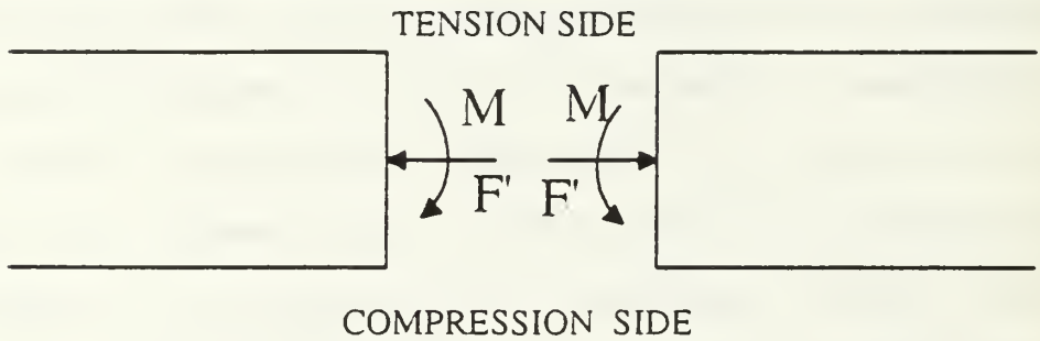
Figure 6a Compressive Force due to Closure
