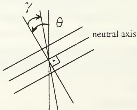
Figure 6b Statically Equivalent Force and Moment
