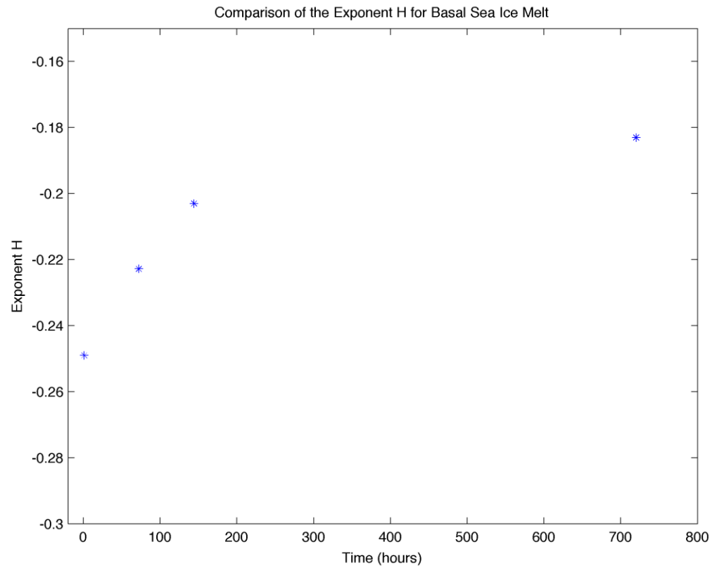
Figure 47. Describes how the exponent H changes over the various temporal averaging methods (1 hour, 3 days, 6 days, and one month). The exponent values increase as the temporal scale increases.
