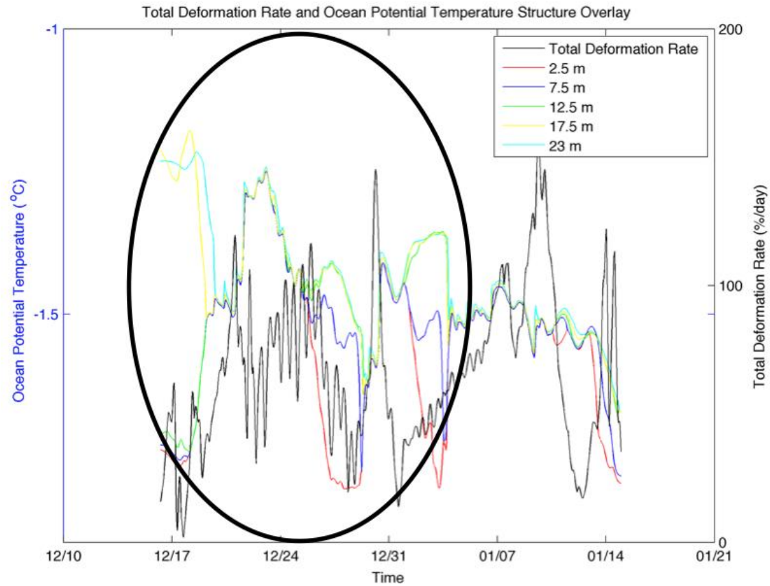
Figure 37. Zoomed in total deformation rate and ocean potential temperature time series overlay (15DEC95–15JAN96). Black oval indicates the event of interest.
