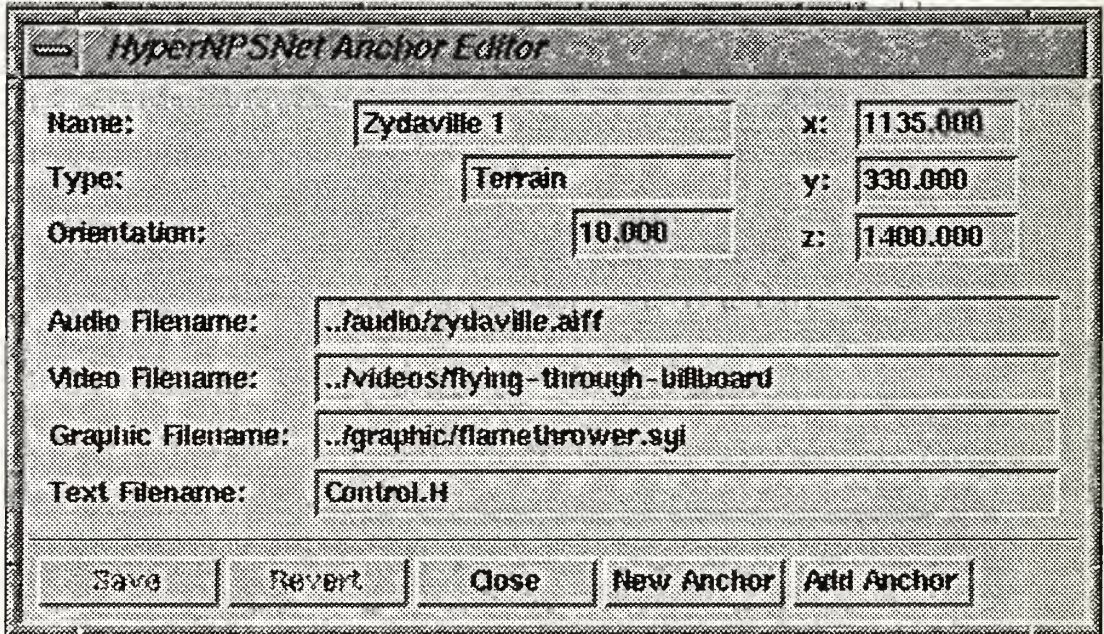
Figure 24: The Anchor Editor Panel
