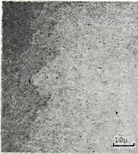
16 repair simulations
