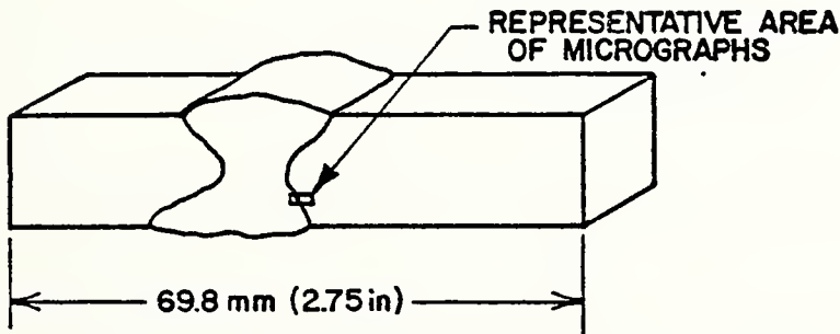
Figure 10. This figure is intended to show the area representing the panorama of micrographs taken of the specimen after etching with the H_3PO_4 solution. The specimen is the same piece as shown in the left side of Figure 9.
