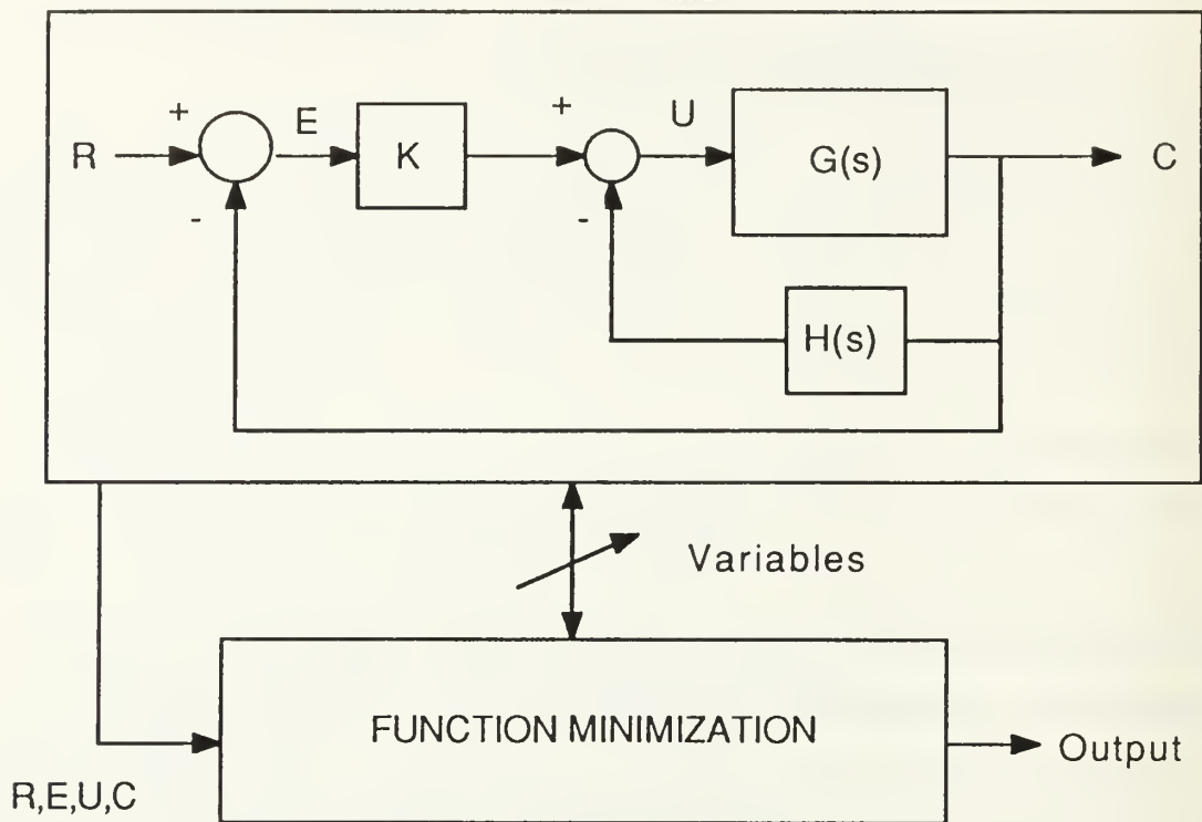
Figure 4. Implementation of function minimization: (From Ref. 1.)
